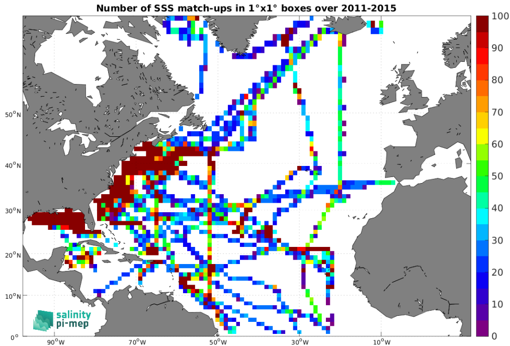
Figure 4: Number of SSS match-ups between TSG (SAMOS) SSS and the Aquarius SSS L3 OR v5 - Monthly (NASA-GSFC) SSS product for the North Atlantic Ocean Pi-MEP region over 1^\circ \times 1^\circ boxes and for the full satellite product period.
