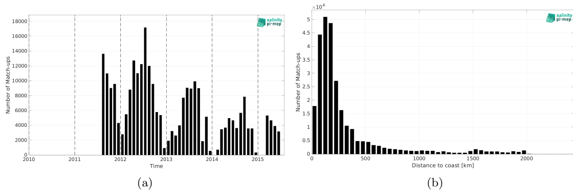
Figure 1: Number of match-ups between TSG (SAMOS) and Aquarius SSS L3 OR v5 - Monthly (NASA-GSFC) SSS as a function of time (a) and as function of the distance to coast (b) over the North Atlantic Ocean Pi-MEP region and for the full satellite product period.
