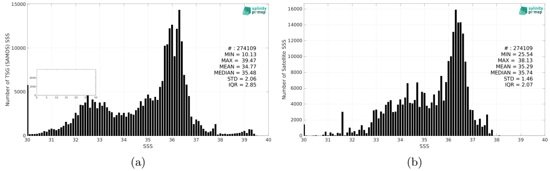
Figure 2: Histograms of SSS from TSG (SAMOS) (a) and Aquarius SSS L3 OR v5 - Monthly (NASA-GSFC) (b) considering all match-up pairs per bins of 0.1 over the North Atlantic Ocean Pi-MEP region and for the full satellite product period.
