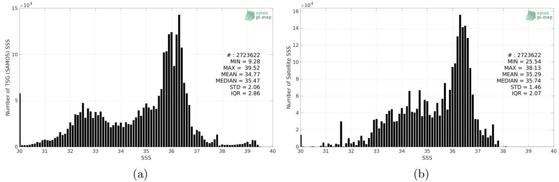
Figure 2: Histograms of SSS from TSG (SAMOS) (a) and Aquarius SSS L3 OR v5 - Monthly (NASA-GSFC) (b) considering all match-up pairs per bins of 0.1 over the North Atlantic Ocean Pi-MEP region and for the full satellite product period.
