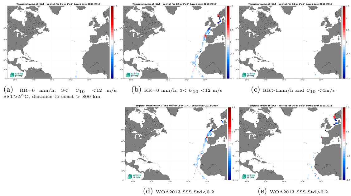
Figure 14: Temporal mean gridded over spatial boxes of size 1^\circ \times 1^\circ of \Delta\text{SSS} (Aquarius SSS L3 OR v5 - Monthly (NASA-GSFC) - TSG (Polarstern)) for 5 different subdatasets corresponding to:RR=0 mm/h, 3 < U_{10} < 12 m/s, SST>5°C, distance to coast > 800 km (a), RR=0 mm/h, 3 < U_{10} < 12 m/s (b), RR>1mm/h and U_{10} < 4 m/s (c), WOA2013 SSS Std<0.2 (d), WOA2013 SSS Std>0.2 (e).
