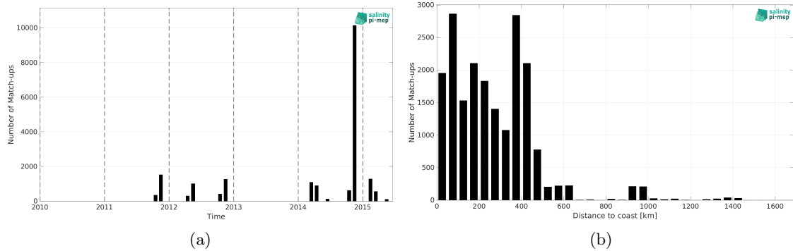
Figure 2: Number of match-ups between TSG (Polarstern) and Aquarius SSS L3 OR v5 - Monthly (NASA-GSFC) SSS as a function of time (a) and as function of the distance to coast (b) over the North Atlantic Ocean Pi-MEP region and for the full satellite product period.
