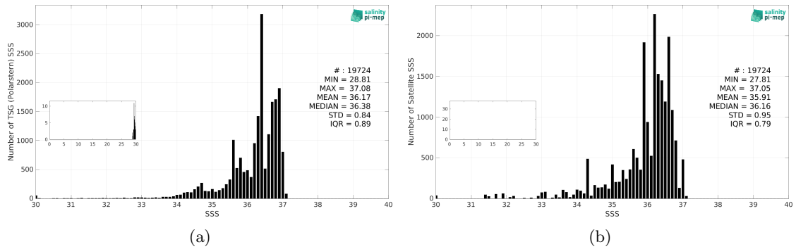
Figure 3: Histograms of SSS from TSG (Polarstern) (a) and Aquarius SSS L3 OR v5 - Monthly (NASA-GSFC) (b) considering all match-up pairs per bins of 0.1 over the North Atlantic Ocean Pi-MEP region and for the full satellite product period.
