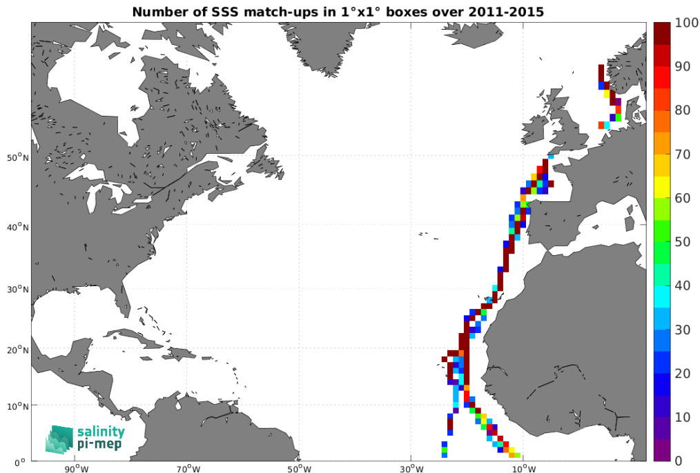
Figure 5: Number of SSS match-ups between TSG (Polarstern) SSS and the Aquarius SSS L3 OR v5 - Monthly (NASA-GSFC) SSS product for the North Atlantic Ocean Pi-MEP region over 1^\circ \times 1^\circ boxes and for the full satellite product period.
