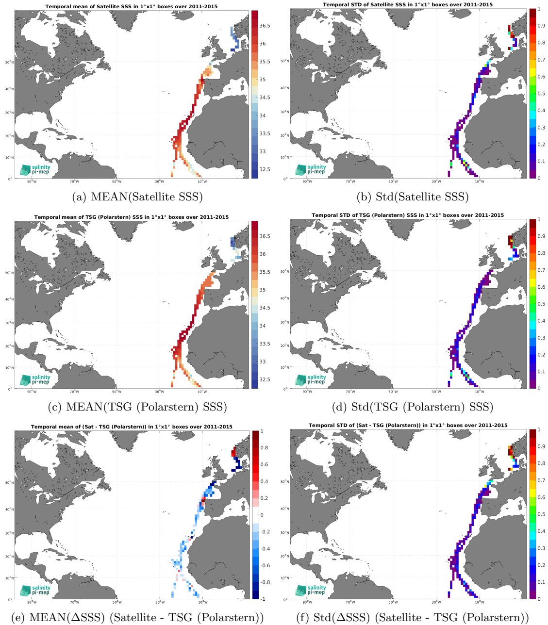
Figure 7: Temporal mean (left) and Std (right) of SSS from Aquarius SSS L3 OR v5 - Monthly (NASA-GSFC) (top), TSG (Polarstern) (middle), and of \Delta SSS (Satellite - TSG (Polarstern)). Only match-up pairs are used to generate these maps.
