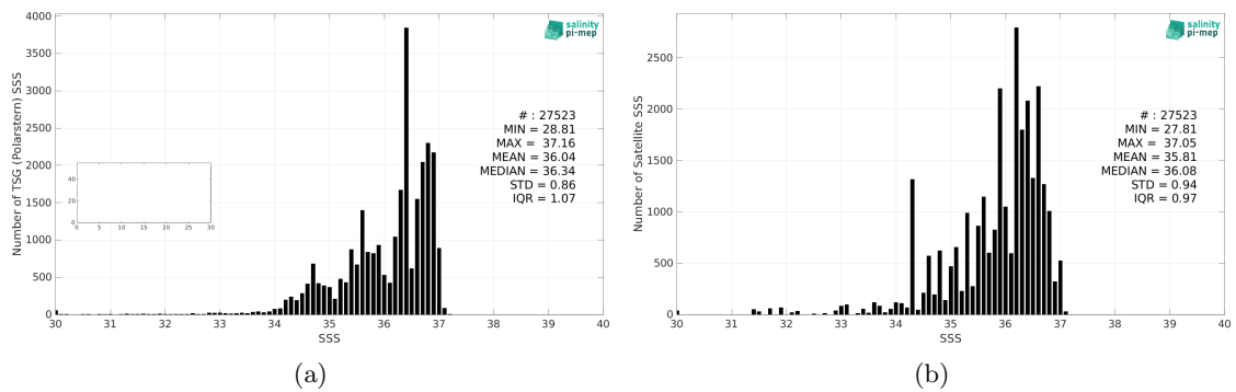
Figure 2: Histograms of SSS from TSG (Polarstern) (a) and Aquarius SSS L3 OR v5 - Monthly (NASA-GSFC) (b) considering all match-up pairs per bins of 0.1 over the North Atlantic Ocean Pi-MEP region and for the full satellite product period.
