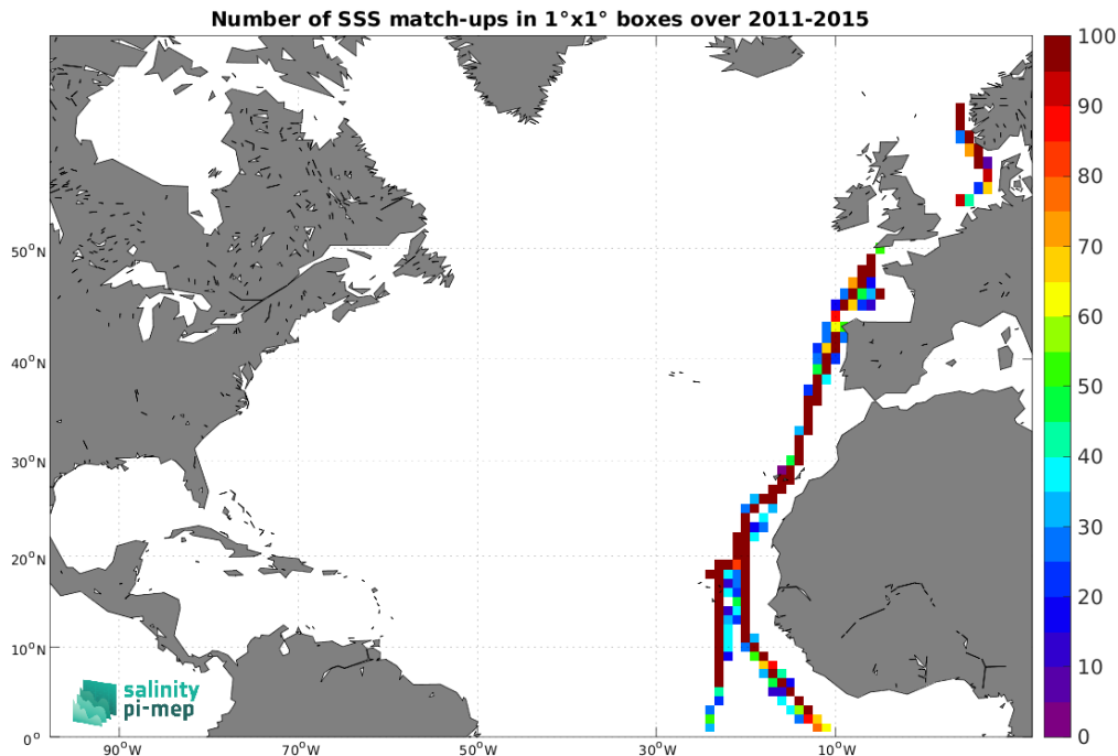
Figure 4: Number of SSS match-ups between TSG (Polarstern) SSS and the Aquarius SSS L3 OR v5 - Monthly (NASA-GSFC) SSS product for the North Atlantic Ocean Pi-MEP region over 1^\circ \times 1^\circ boxes and for the full satellite product period.
