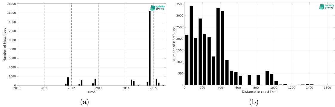
Figure 1: Number of match-ups between TSG (Polarstern) and Aquarius SSS L3 OR v5 - Monthly (NASA-GSFC) SSS as a function of time (a) and as function of the distance to coast (b) over the North Atlantic Ocean Pi-MEP region and for the full satellite product period.
