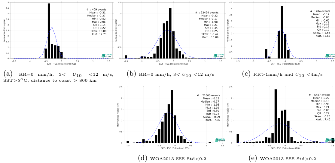
Figure 13: Normalized histogram of \Delta\text{SSS} (Aquarius SSS L3 OR v5 - Monthly (NASA-GSFC) - TSG (Polarstern)) for 5 different subdatasets corresponding to: RR=0 mm/h, 3 < U_{10} < 12 m/s, SST > 5^\circ\text{C} , distance to coast > 800 km (a), RR=0 mm/h, 3 < U_{10} < 12 m/s (b), RR > 1 mm/h and U_{10} < 4 m/s (c), WOA2013 SSS Std < 0.2 (d), WOA2013 SSS Std > 0.2 (e).
