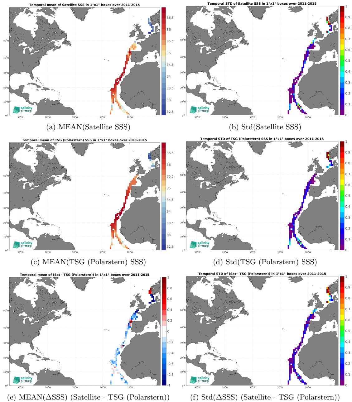
Figure 6: Temporal mean (left) and Std (right) of SSS from Aquarius SSS L3 OR v5 - Monthly (NASA-GSFC) (top), TSG (Polarstern) (middle), and of \Delta SSS (Satellite - TSG (Polarstern)). Only match-up pairs are used to generate these maps.
