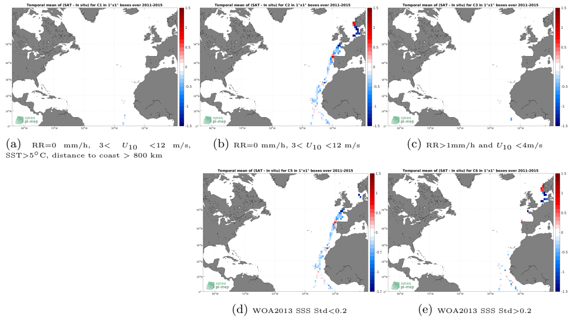
Figure 12: Temporal mean gridded over spatial boxes of size 1^\circ \times 1^\circ of \Delta\text{SSS} (Aquarius SSS L3 OR v5 - Monthly (NASA-GSFC) - TSG (Polarstern)) for 5 different subdatasets corresponding to:RR=0 mm/h, 3 < U_{10} < 12 m/s, SST >5^\circ\text{C} , distance to coast > 800 km (a), RR=0 mm/h, 3 < U_{10} < 12 m/s (b), RR >1 mm/h and U_{10} < 4 m/s (c), WOA2013 SSS Std <0.2 (d), WOA2013 SSS Std >0.2 (e).
