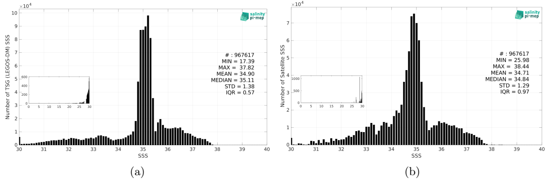
Figure 3: Histograms of SSS from TSG (LEGOS-DM) (a) and Aquarius SSS L3 OR v5 - Monthly (NASA-GSFC) (b) considering all match-up pairs per bins of 0.1 over the North Atlantic Ocean Pi-MEP region and for the full satellite product period.
