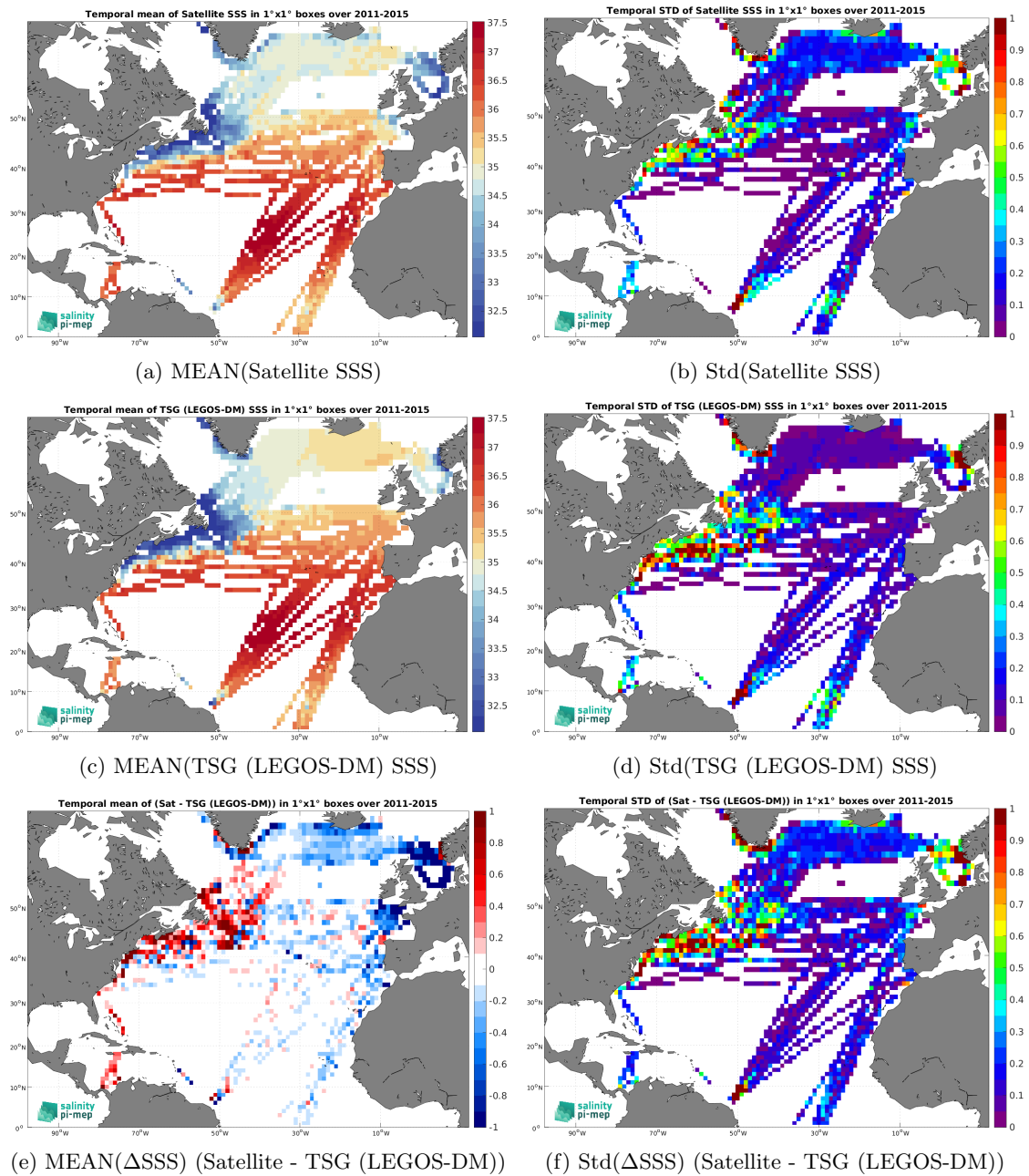
Figure 7: Temporal mean (left) and Std (right) of SSS from Aquarius SSS L3 OR v5 - Monthly (NASA-GSFC) (top), TSG (LEGOS-DM) (middle), and of \Delta SSS (Satellite - TSG (LEGOS-DM)). Only match-up pairs are used to generate these maps.
