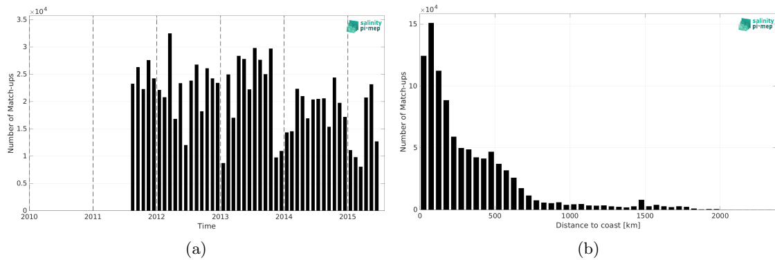
Figure 2: Number of match-ups between TSG (LEGOS-DM) and Aquarius SSS L3 OR v5 - Monthly (NASA-GSFC) SSS as a function of time (a) and as function of the distance to coast (b) over the North Atlantic Ocean Pi-MEP region and for the full satellite product period.
