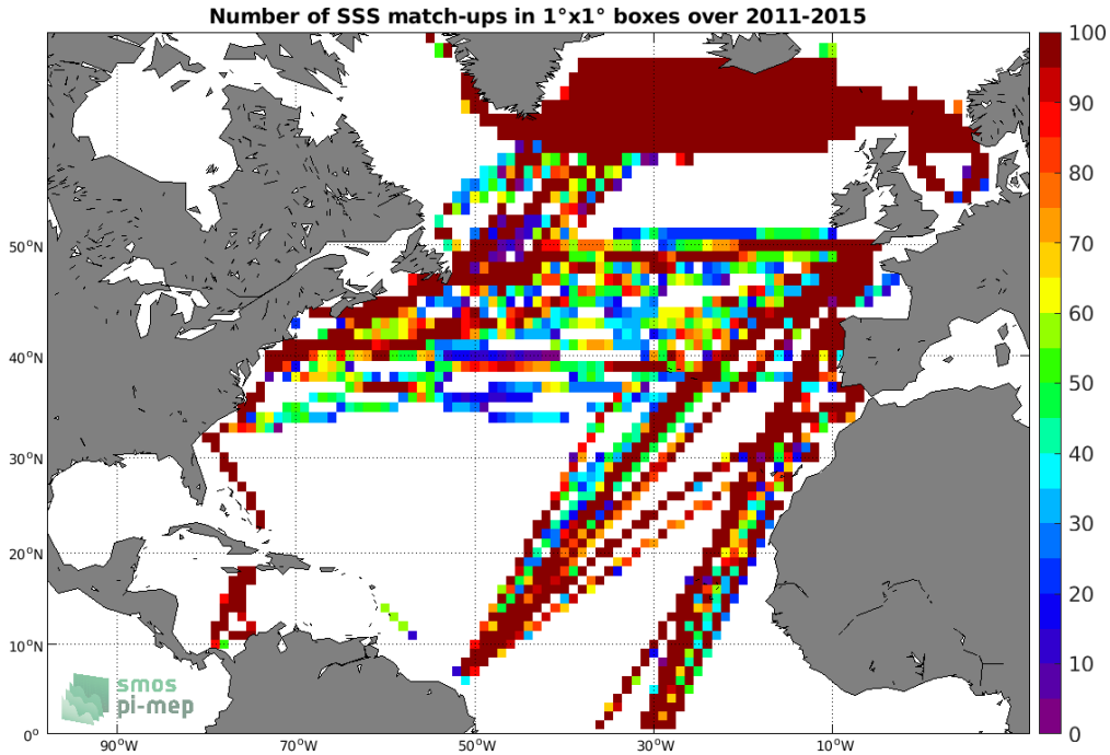
Figure 4: Number of SSS match-ups between TSG (LEGOS-DM) SSS and the Aquarius SSS L3 OR v5 - Monthly (NASA-GSFC) SSS product for the North Atlantic Ocean Pi-MEP region over 1°x1° boxes and for the full satellite product period.
