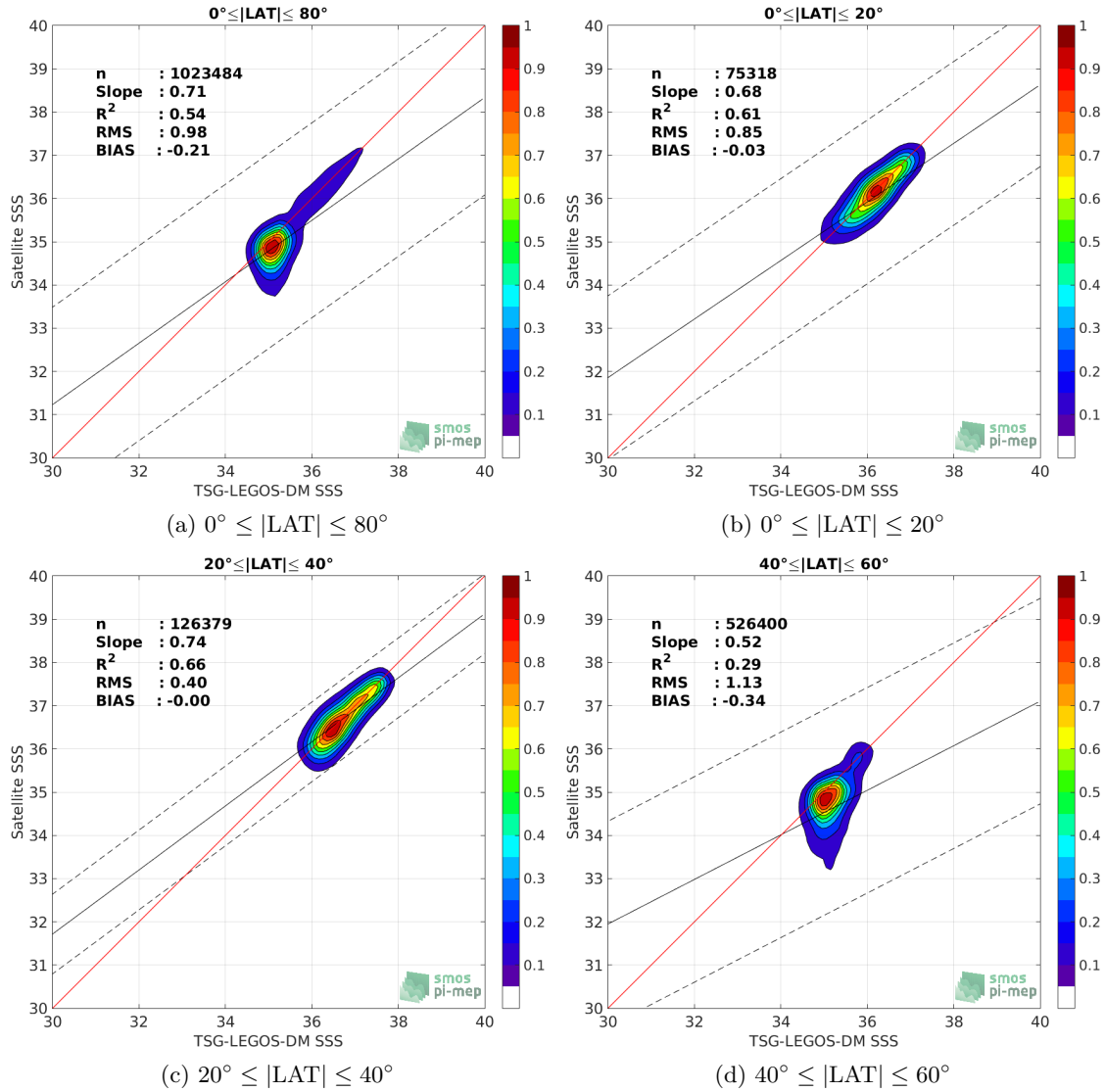
Figure 9: Contour maps of the concentration of Aquarius-L3-OR-V5-MONTHLY-1DEG SSS (y-axis) versus TSG-LEGOS-DM SSS (x-axis) at match-up pairs for different latitude bands. For each plot, the red line shows x=y . The black thin and dashed lines indicate a linear fit through the data cloud and the \pm 95\% confidence levels, respectively. The number match-up pairs n , the slope and R^2 coefficient of the linear fit, the root mean square (RMS) and the mean bias between satellite and in situ data are indicated for each latitude band in each plots.
