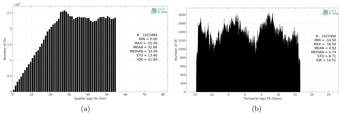
Figure 5: Histograms of the spatial (a) and temporal (b) lags between the time of the TSG-LEGOS-DM measurements and the date of the corresponding Aquarius-L3-OR-V5-MONTHLY-1DEG SSS product.
