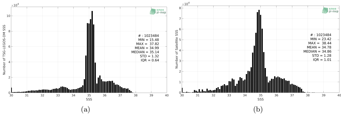
Figure 2: Histograms of SSS from TSG-LEGOS-DM (a) and Aquarius-L3-OR-V5-MONTHLY-1DEG (b) considering all match-up pairs per bins of 0.1 over the North Atlantic Ocean Pi-MEP region and for the full satellite product period.
