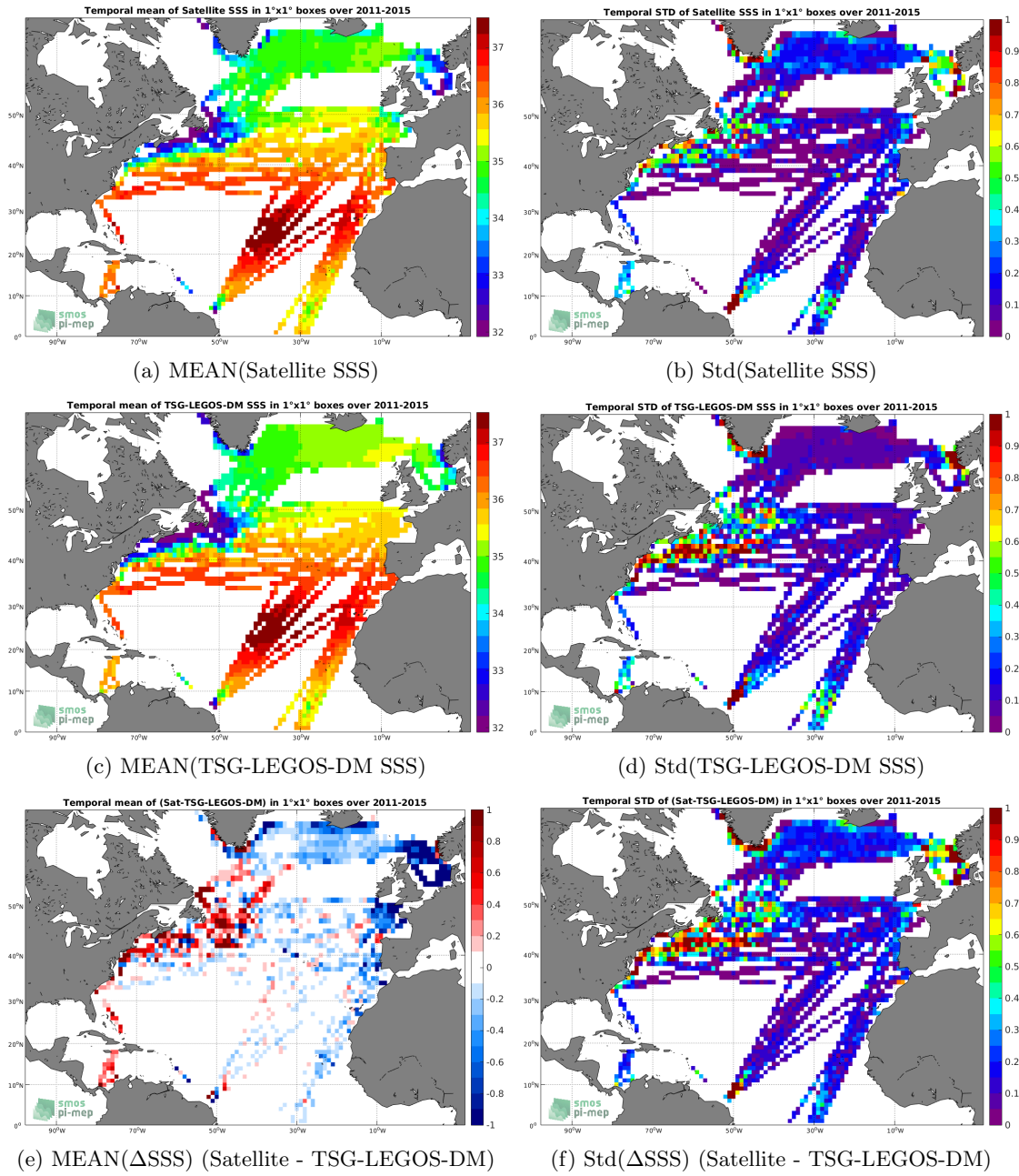
Figure 6: Temporal mean (left) and Std (right) of SSS from Aquarius-L3-OR-V5-MONTHLY-1DEG (top), TSG-LEGOS-DM (middle), and of \Delta SSS (Satellite - TSG-LEGOS-DM). Only match-up pairs are used to generate these maps.
