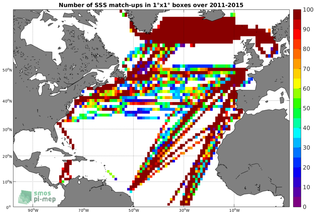
Figure 4: Number of SSS match-ups between TSG-LEGOS-DM SSS and the Aquarius-L3-OR-V5-MONTHLY-1DEG SSS product for the North Atlantic Ocean Pi-MEP region over 1^\circ \times 1^\circ boxes and for the full satellite product period.
