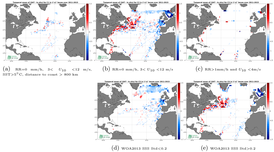
Figure 12: Temporal mean gridded over spatial boxes of size 1^\circ \times 1^\circ of \Delta SSS (Aquarius-L3-OR-V5-MONTHLY-1DEG - TSG-LEGOS-DM) for 5 different subdatasets corresponding to:RR=0 mm/h, 3 < U_{10} < 12 m/s, SST >5^\circ C, distance to coast > 800 km (a), RR=0 mm/h, 3 < U_{10} < 12 m/s (b), RR >1 mm/h and U_{10} < 4 m/s (c), WOA2013 SSS Std <0.2 (d), WOA2013 SSS Std >0.2 (e).
