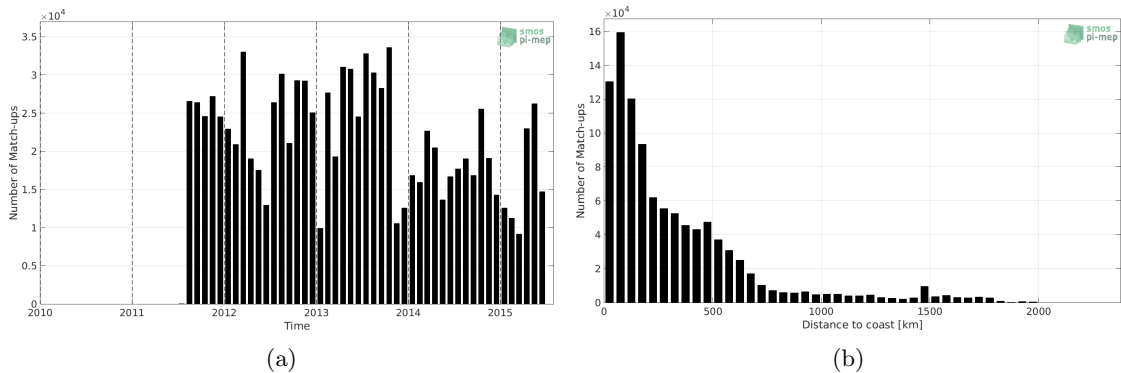
Figure 1: Number of match-ups between TSG-LEGOS-DM and Aquarius-L3-OR-V5-MONTHLY-1DEG SSS as a function of time (a) and as function of the distance to coast (b) over the North Atlantic Ocean Pi-MEP region and for the full satellite product period.
