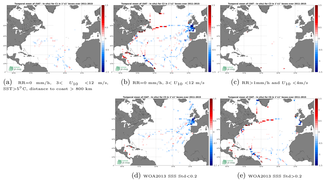
Figure 12: Temporal mean gridded over spatial boxes of size 1^\circ \times 1^\circ of \Delta\text{SSS} (Aquarius SSS L3 OR v5 - Monthly (NASA-GSFC) - TSG (GOSUD-Sailing-ship)) for 5 different subdatasets corresponding to: RR=0 mm/h, 3 < U_{10} < 12 m/s, SST > 5°C, distance to coast > 800 km (a), RR=0 mm/h, 3 < U_{10} < 12 m/s (b), RR > 1mm/h and U_{10} < 4 m/s (c), WOA2013 SSS Std < 0.2 (d), WOA2013 SSS Std > 0.2 (e).
