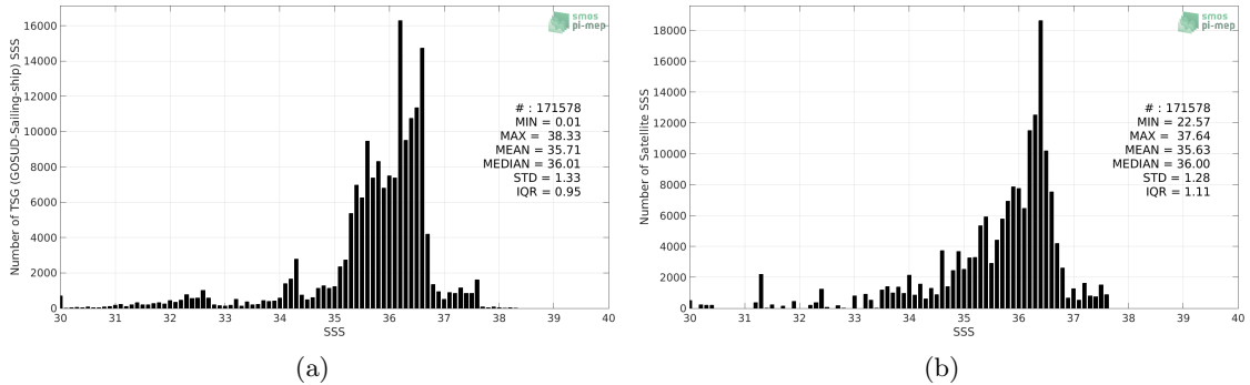
Figure 2: Histograms of SSS from TSG (GOSUD-Sailing-ship) (a) and Aquarius SSS L3 OR v5 - Monthly (NASA-GSFC) (b) considering all match-up pairs per bins of 0.1 over the North Atlantic Ocean Pi-MEP region and for the full satellite product period.
