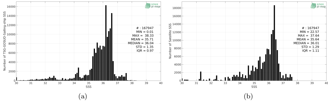
Figure 2: Histograms of SSS from TSG-GOSUD-Sailing-ship (a) and Aquarius-L3-OR-V5-MONTHLY-1DEG (b) considering all match-up pairs per bins of 0.1 over the North Atlantic Ocean Pi-MEP region and for the full satellite product period.
