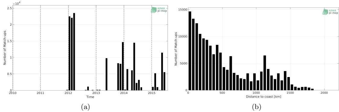
Figure 1: Number of match-ups between TSG-GOSUD-Sailing-ship and Aquarius-L3-OR-V5-MONTHLY-1DEG SSS as a function of time (a) and as function of the distance to coast (b) over the North Atlantic Ocean Pi-MEP region and for the full satellite product period.
