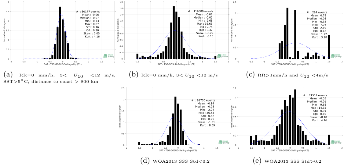
Figure 13: Normalized histogram of \Delta\text{SSS} (Aquarius-L3-OR-V5-MONTHLY-1DEG - TSG-GOSUD-Sailing-ship) for 5 different subdatasets corresponding to: RR=0 mm/h, 3 < U_{10} < 12 m/s, SST >5^{\circ}\text{C} , distance to coast > 800 km (a), RR=0 mm/h, 3 < U_{10} < 12 m/s (b), RR >1 mm/h and U_{10} < 4 m/s (c), WOA2013 SSS Std <0.2 (d), WOA2013 SSS Std >0.2 (e).
