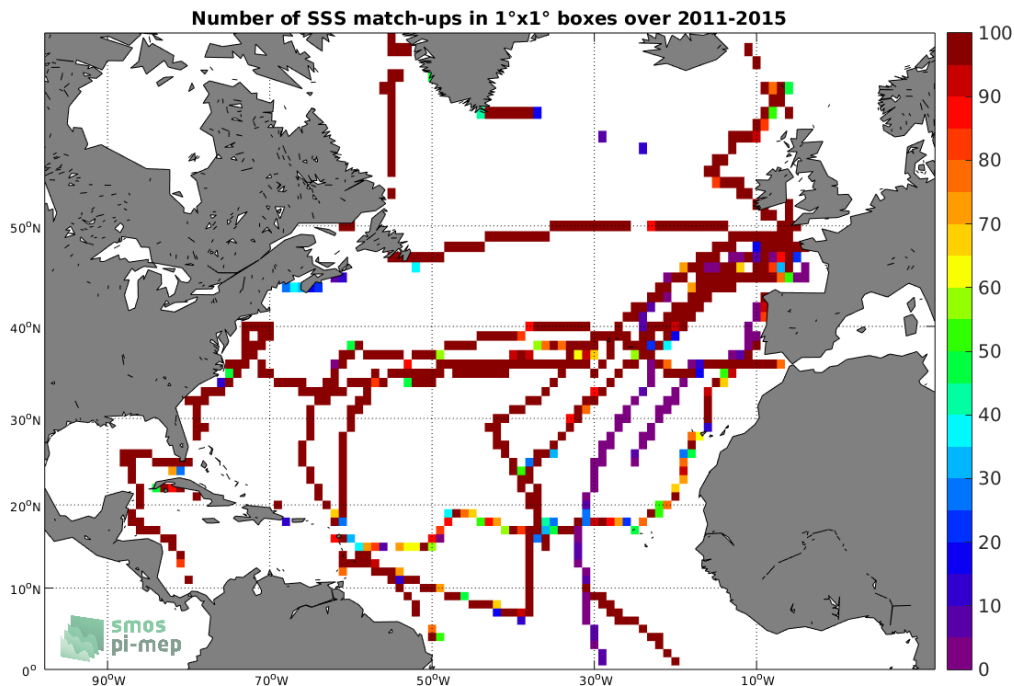
Figure 4: Number of SSS match-ups between TSG-GOSUD-Sailing-ship SSS and the Aquarius-L3-OR-V5-MONTHLY-1DEG SSS product for the North Atlantic Ocean Pi-MEP region over 1^\circ \times 1^\circ boxes and for the full satellite product period.
