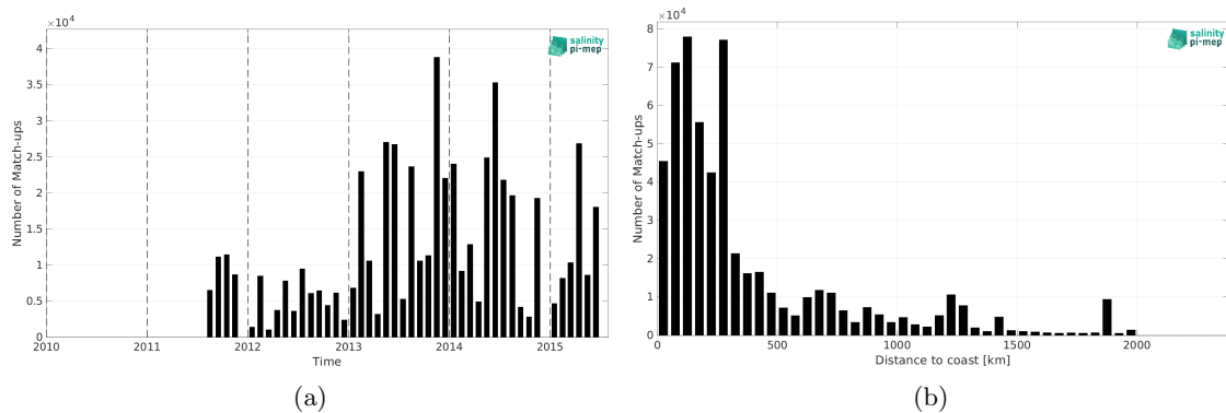
Figure 2: Number of match-ups between TSG (GOSUD-Research-vessel) and Aquarius SSS L3 OR v5 - Monthly (NASA-GSFC) SSS as a function of time (a) and as function of the distance to coast (b) over the North Atlantic Ocean Pi-MEP region and for the full satellite product period.
