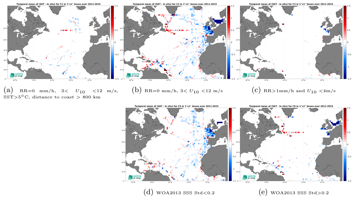
Figure 14: Temporal mean gridded over spatial boxes of size 1^\circ \times 1^\circ of \Delta\text{SSS} (Aquarius SSS L3 OR v5 - Monthly (NASA-GSFC) - TSG (GOSUD-Research-vessel)) for 5 different subdatasets corresponding to:RR=0 mm/h, 3 < U_{10} < 12 m/s, SST > 5°C, distance to coast > 800 km (a), RR=0 mm/h, 3 < U_{10} < 12 m/s (b), RR > 1mm/h and U_{10} < 4 m/s (c), WOA2013 SSS Std < 0.2 (d), WOA2013 SSS Std > 0.2 (e).
