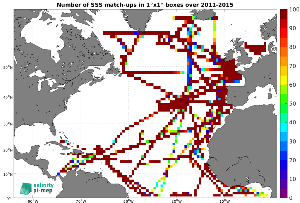
Figure 5: Number of SSS match-ups between TSG (GOSUD-Research-vessel) SSS and the Aquarius SSS L3 OR v5 - Monthly (NASA-GSFC) SSS product for the North Atlantic Ocean Pi-MEP region over 1^\circ \times 1^\circ boxes and for the full satellite product period.
