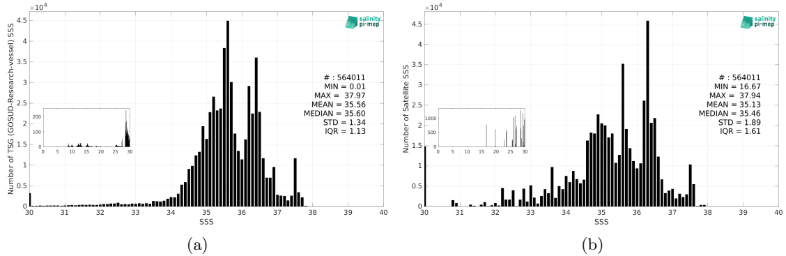
Figure 3: Histograms of SSS from TSG (GOSUD-Research-vessel) (a) and Aquarius SSS L3 OR v5 - Monthly (NASA-GSFC) (b) considering all match-up pairs per bins of 0.1 over the North Atlantic Ocean Pi-MEP region and for the full satellite product period.
