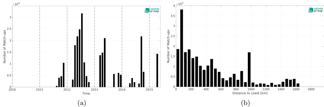
Figure 2: Number of match-ups between TSG (CSIC-UTM) and Aquarius SSS L3 OR v5 - Monthly (NASA-GSFC) SSS as a function of time (a) and as function of the distance to coast (b) over the North Atlantic Ocean Pi-MEP region and for the full satellite product period.
