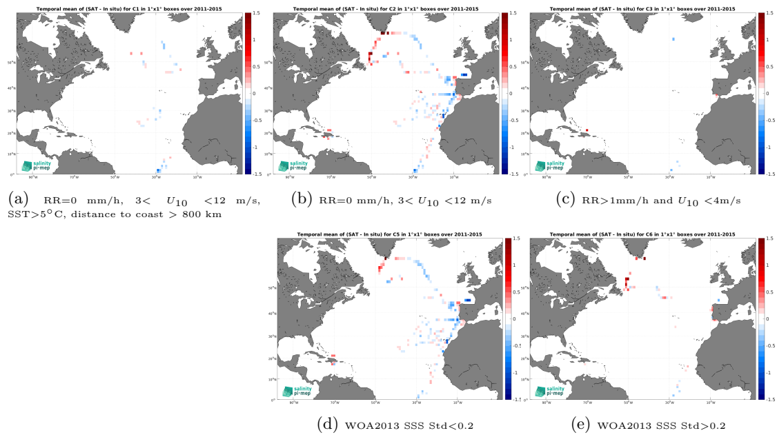
Figure 14: Temporal mean gridded over spatial boxes of size 1^\circ \times 1^\circ of \Delta\text{SSS} (Aquarius SSS L3 OR v5 - Monthly (NASA-GSFC) - TSG (CSIC-UTM)) for 5 different subdatasets corresponding to:RR=0 mm/h, 3 < U_{10} < 12 m/s, SST > 5°C, distance to coast > 800 km (a), RR=0 mm/h, 3 < U_{10} < 12 m/s (b), RR > 1mm/h and U_{10} < 4 m/s (c), WOA2013 SSS Std < 0.2 (d), WOA2013 SSS Std > 0.2 (e).
