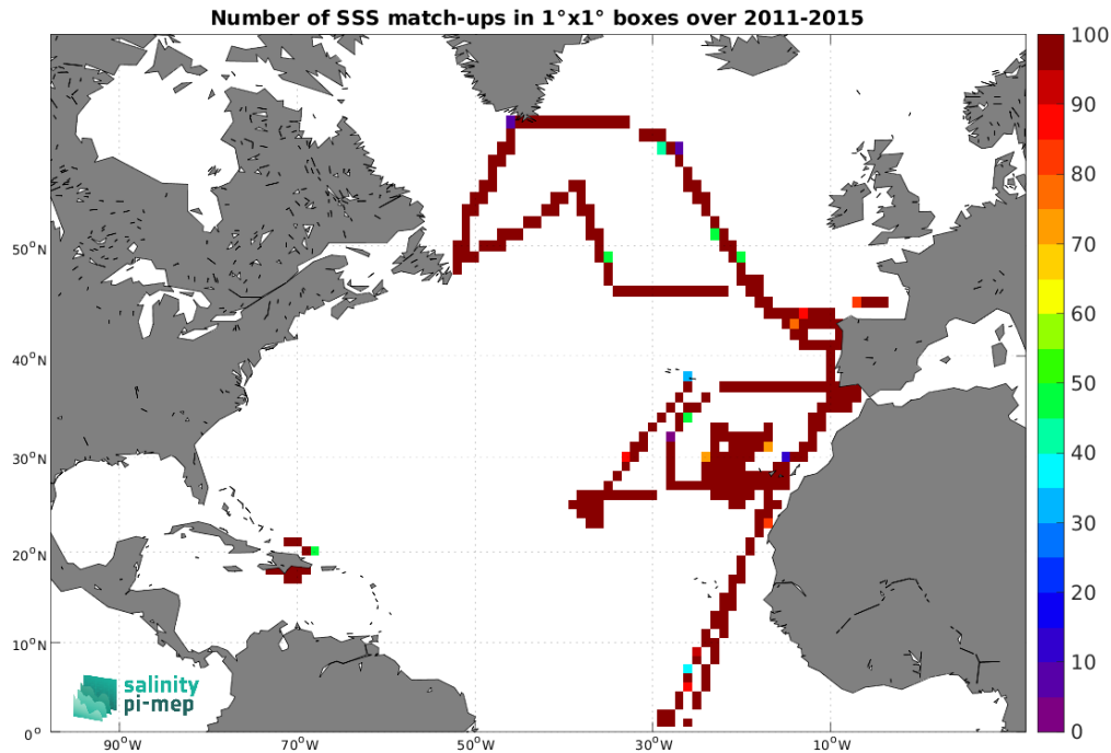
Figure 5: Number of SSS match-ups between TSG (CSIC-UTM) SSS and the Aquarius SSS L3 OR v5 - Monthly (NASA-GSFC) SSS product for the North Atlantic Ocean Pi-MEP region over 1^\circ \times 1^\circ boxes and for the full satellite product period.
