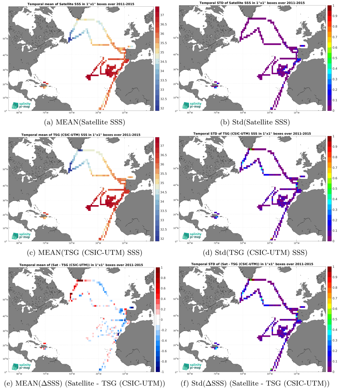
Figure 7: Temporal mean (left) and Std (right) of SSS from Aquarius SSS L3 OR v5 - Monthly (NASA-GSFC) (top), TSG (CSIC-UTM) (middle), and of \Delta SSS (Satellite - TSG (CSIC-UTM)). Only match-up pairs are used to generate these maps.
