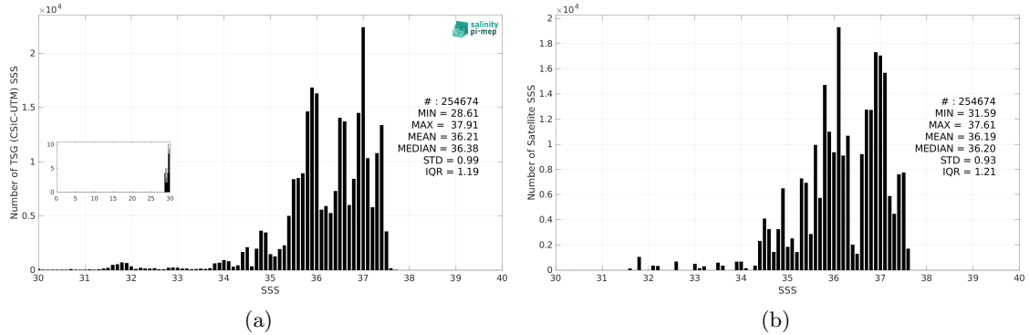
Figure 3: Histograms of SSS from TSG (CSIC-UTM) (a) and Aquarius SSS L3 OR v5 - Monthly (NASA-GSFC) (b) considering all match-up pairs per bins of 0.1 over the North Atlantic Ocean Pi-MEP region and for the full satellite product period.
