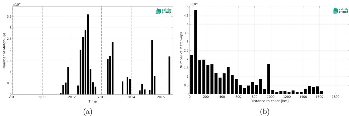
Figure 1: Number of match-ups between TSG (CSIC-UTM) and Aquarius SSS L3 OR v5 - Monthly (NASA-GSFC) SSS as a function of time (a) and as function of the distance to coast (b) over the North Atlantic Ocean Pi-MEP region and for the full satellite product period.
