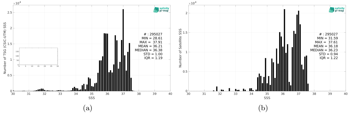
Figure 2: Histograms of SSS from TSG (CSIC-UTM) (a) and Aquarius SSS L3 OR v5 - Monthly (NASA-GSFC) (b) considering all match-up pairs per bins of 0.1 over the North Atlantic Ocean Pi-MEP region and for the full satellite product period.
