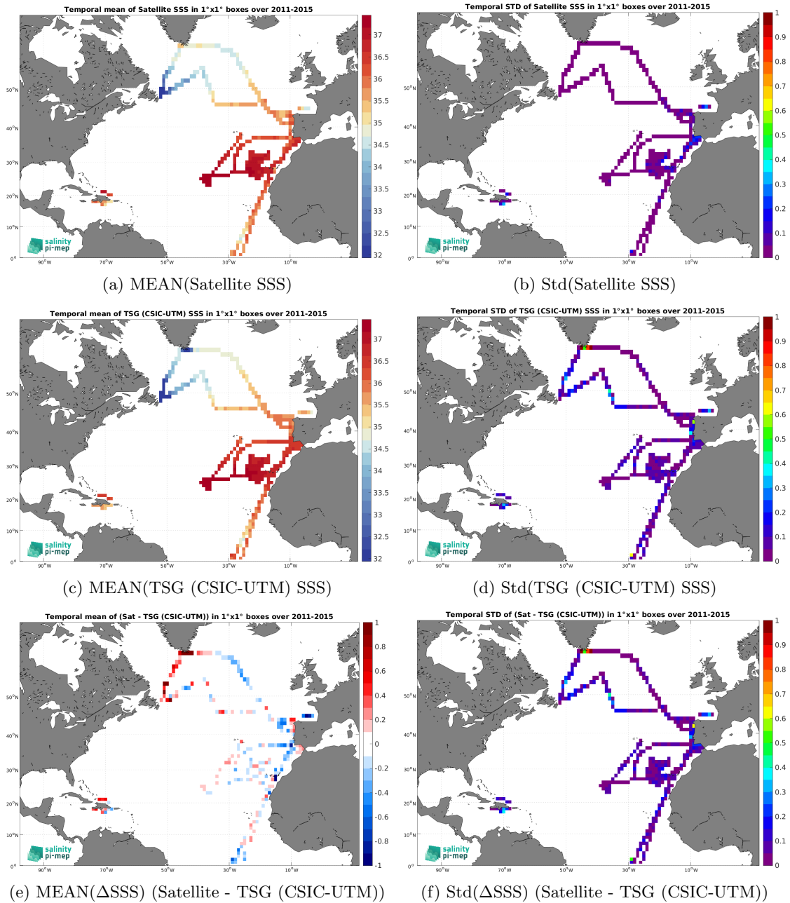
Figure 6: Temporal mean (left) and Std (right) of SSS from Aquarius SSS L3 OR v5 - Monthly (NASA-GSFC) (top), TSG (CSIC-UTM) (middle), and of \Delta SSS (Satellite - TSG (CSIC-UTM)). Only match-up pairs are used to generate these maps.
