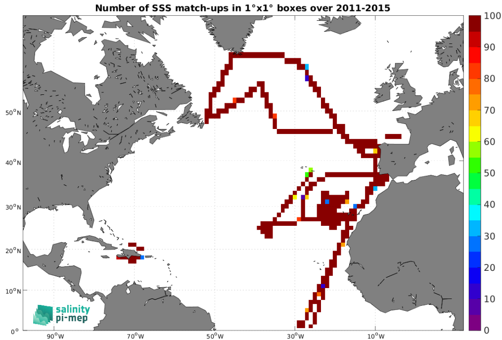
Figure 4: Number of SSS match-ups between TSG (CSIC-UTM) SSS and the Aquarius SSS L3 OR v5 - Monthly (NASA-GSFC) SSS product for the North Atlantic Ocean Pi-MEP region over 1^\circ \times 1^\circ boxes and for the full satellite product period.
