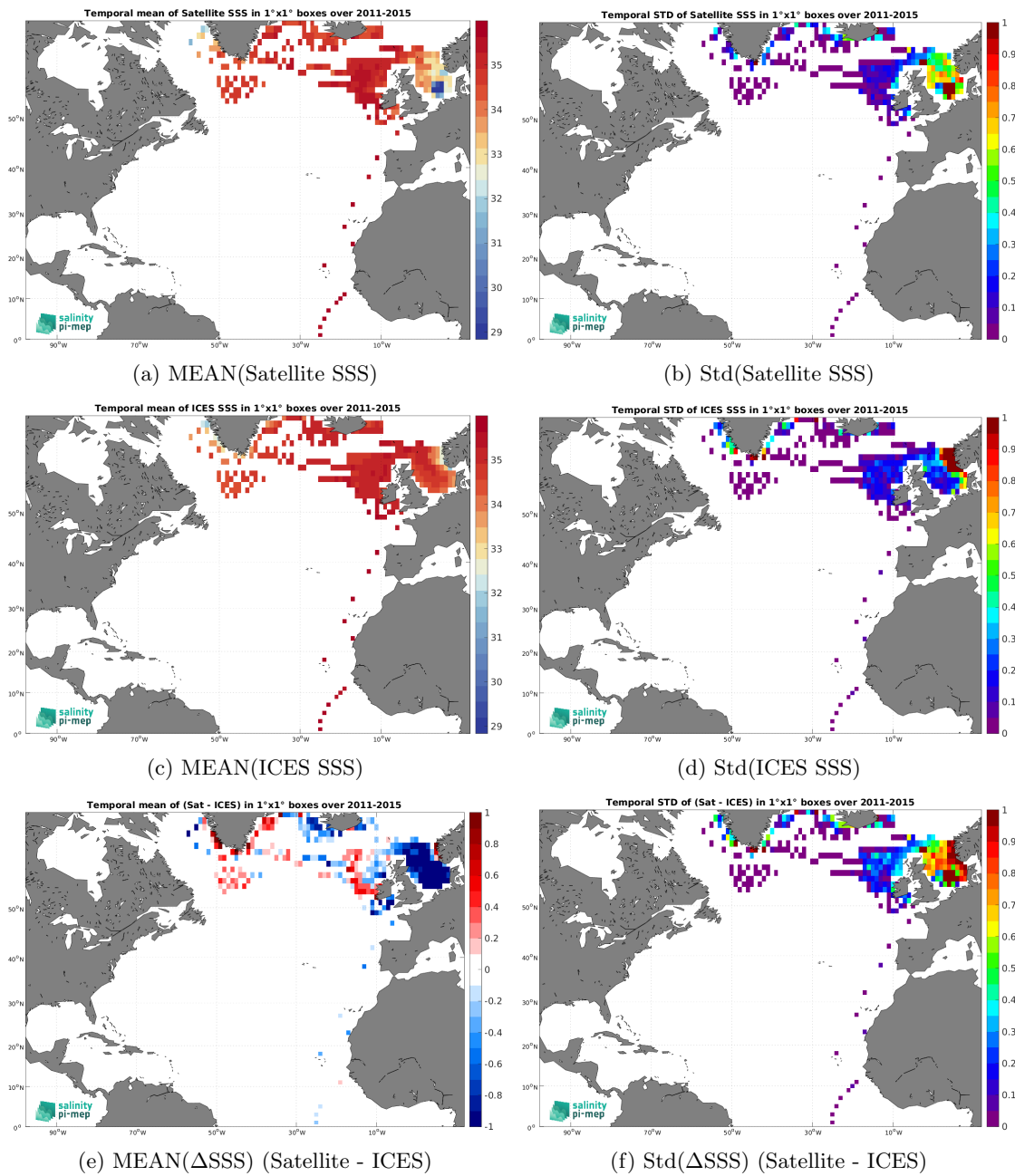
Figure 7: Temporal mean (left) and Std (right) of SSS from Aquarius SSS L3 OR v5 - Monthly (NASA-GSFC) (top), ICES (middle), and of \Delta SSS (Satellite - ICES). Only match-up pairs are used to generate these maps.
