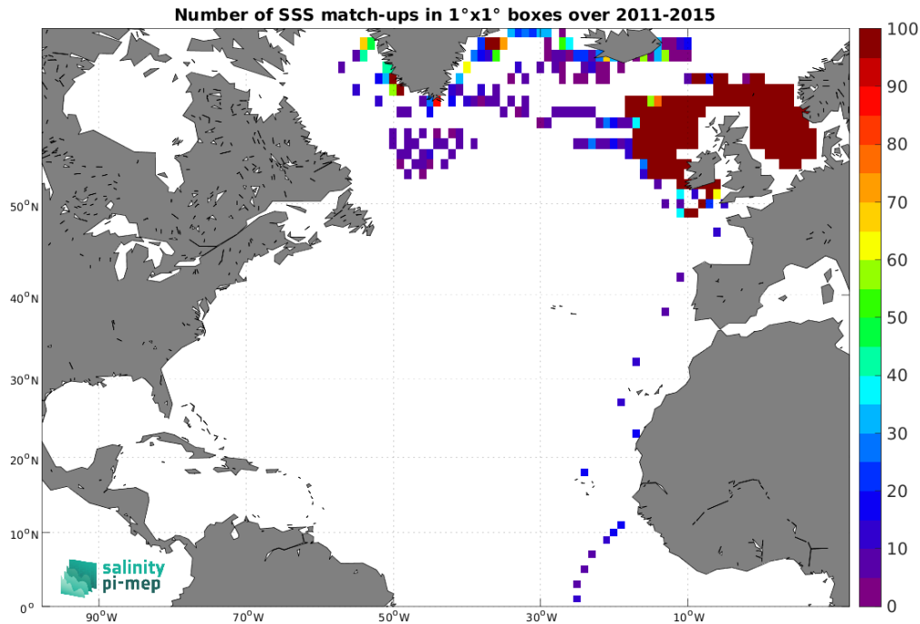
Figure 5: Number of SSS match-ups between ICES SSS and the Aquarius SSS L3 OR v5 - Monthly (NASA-GSFC) SSS product for the North Atlantic Ocean Pi-MEP region over 1^\circ \times 1^\circ boxes and for the full satellite product period.
