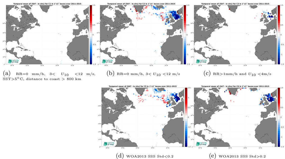
Figure 14: Temporal mean gridded over spatial boxes of size 1^\circ \times 1^\circ of \Delta SSS (Aquarius SSS L3 OR v5 - Monthly (NASA-GSFC) - ICES) for 5 different subdatasets corresponding to:RR=0 mm/h, 3 < U_{10} < 12 m/s, SST >5^\circ\text{C} , distance to coast > 800 km (a), RR=0 mm/h, 3 < U_{10} < 12 m/s (b), RR >1 mm/h and U_{10} < 4 m/s (c), WOA2013 SSS Std <0.2 (d), WOA2013 SSS Std >0.2 (e).
