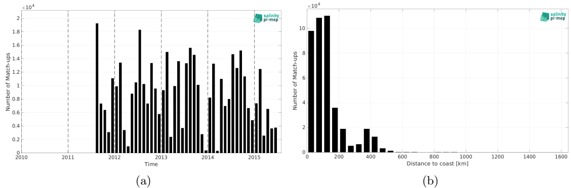
Figure 2: Number of match-ups between ICES and Aquarius SSS L3 OR v5 - Monthly (NASA-GSFC) SSS as a function of time (a) and as function of the distance to coast (b) over the North Atlantic Ocean Pi-MEP region and for the full satellite product period.
