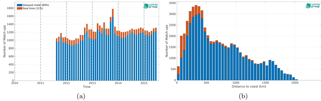
Figure 1: Number of match-ups between Argo and Aquarius SSS L3 OR v5 - Monthly (NASA-GSFC) SSS as a function of time (a) and as function of the distance to coast (b) over the North Atlantic Ocean Pi-MEP region and for the full satellite product period.
