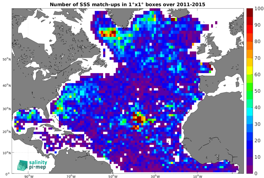
Figure 4: Number of SSS match-ups between Argo SSS and the Aquarius SSS L3 OR v5 - Monthly (NASA-GSFC) SSS product for the North Atlantic Ocean Pi-MEP region over 1^\circ \times 1^\circ boxes and for the full satellite product period.
