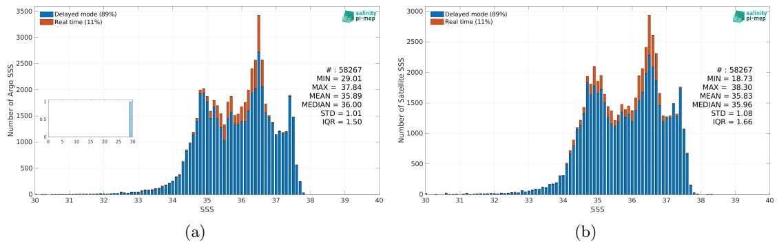
Figure 2: Histograms of SSS from Argo (a) and Aquarius SSS L3 OR v5 - Monthly (NASA-GSFC) (b) considering all match-up pairs per bins of 0.1 over the North Atlantic Ocean Pi-MEP region and for the full satellite product period.
