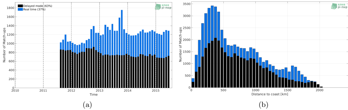
Figure 1: Number of match-ups between Argo and Aquarius-L3-OR-V5-MONTHLY-1DEG SSS as a function of time (a) and as function of the distance to coast (b) over the North Atlantic Ocean Pi-MEP region and for the full satellite product period.
