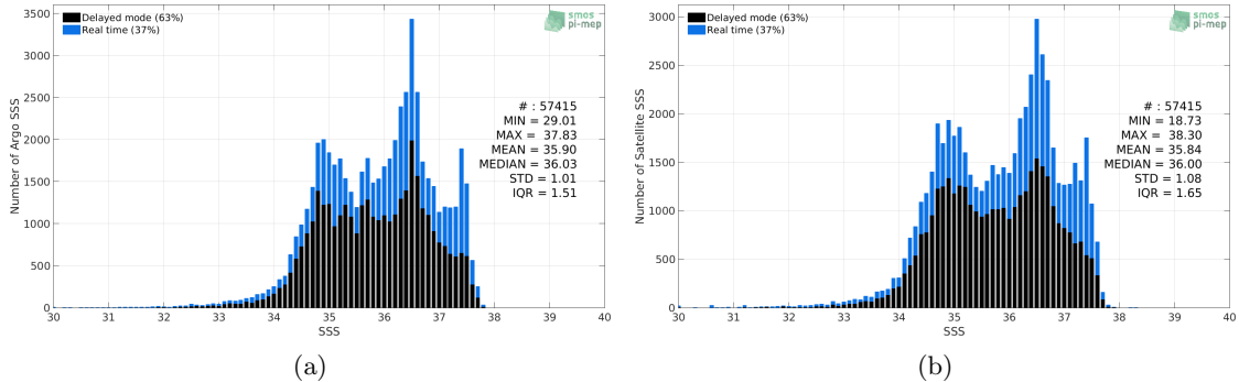
Figure 2: Histograms of SSS from Argo (a) and Aquarius-L3-OR-V5-MONTHLY-1DEG (b) considering all match-up pairs per bins of 0.1 over the North Atlantic Ocean Pi-MEP region and for the full satellite product period.
