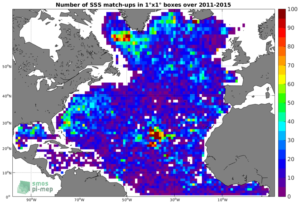
Figure 4: Number of SSS match-ups between Argo SSS and the Aquarius-L3-OR-V5-MONTHLY-1DEG SSS product for the North Atlantic Ocean Pi-MEP region over 1°x1° boxes and for the full satellite product period.
