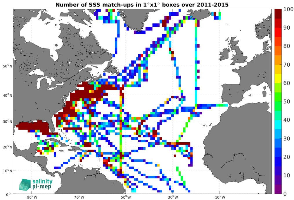
Figure 5: Number of SSS match-ups between TSG (SAMOS) SSS and the Aquarius SSS L3 OR v5 - Monthly - Rain mask (NASA-GSFC) SSS product for the North Atlantic Ocean Pi-MEP region over 1^\circ \times 1^\circ boxes and for the full satellite product period.
