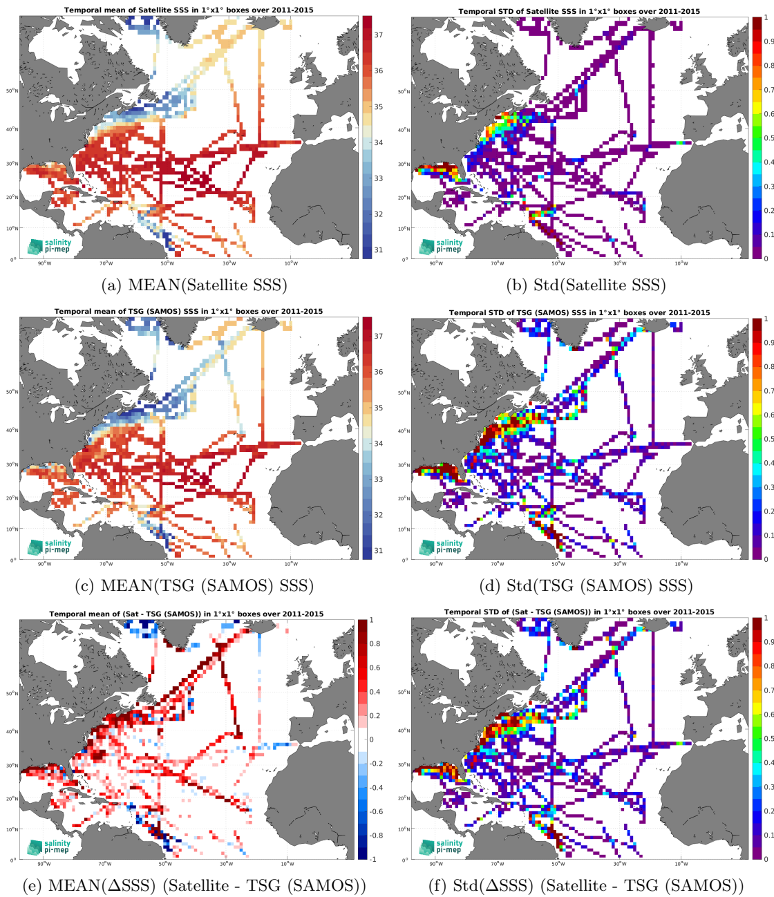
Figure 7: Temporal mean (left) and Std (right) of SSS from Aquarius SSS L3 OR v5 - Monthly - Rain mask (NASA-GSFC) (top), TSG (SAMOS) (middle), and of \Delta SSS (Satellite - TSG (SAMOS)). Only match-up pairs are used to generate these maps.
