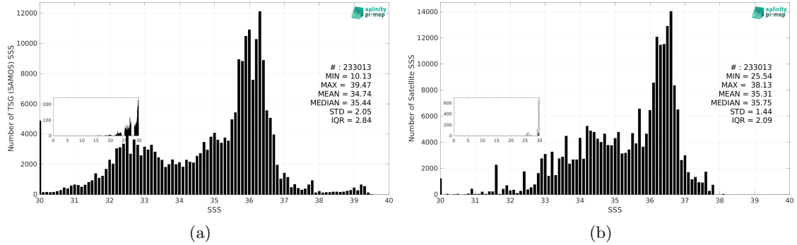
Figure 3: Histograms of SSS from TSG (SAMOS) (a) and Aquarius SSS L3 OR v5 - Monthly - Rain mask (NASA-GSFC) (b) considering all match-up pairs per bins of 0.1 over the North Atlantic Ocean Pi-MEP region and for the full satellite product period.
