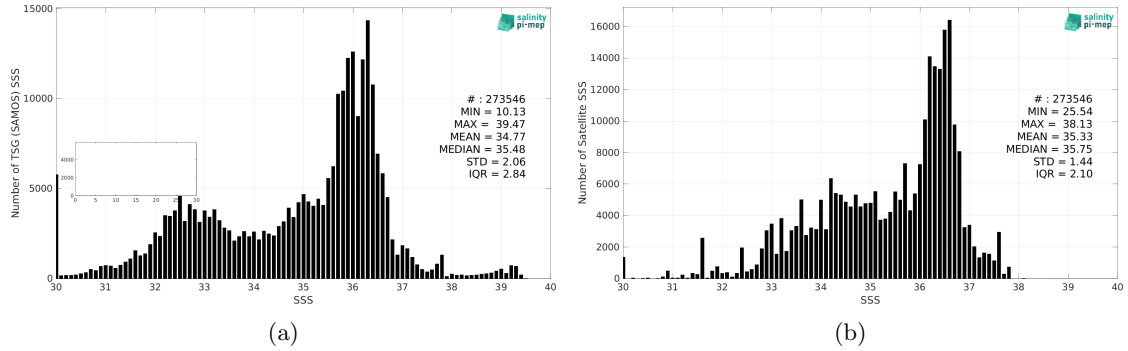
Figure 2: Histograms of SSS from TSG (SAMOS) (a) and Aquarius SSS L3 OR v5 - Monthly - Rain mask (NASA-GSFC) (b) considering all match-up pairs per bins of 0.1 over the North Atlantic Ocean Pi-MEP region and for the full satellite product period.
