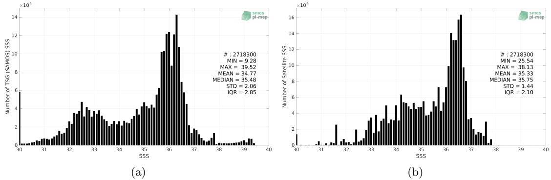
Figure 2: Histograms of SSS from TSG (SAMOS) (a) and Aquarius SSS L3 OR v5 - Monthly - Rain mask (NASA-GSFC) (b) considering all match-up pairs per bins of 0.1 over the North Atlantic Ocean Pi-MEP region and for the full satellite product period.
