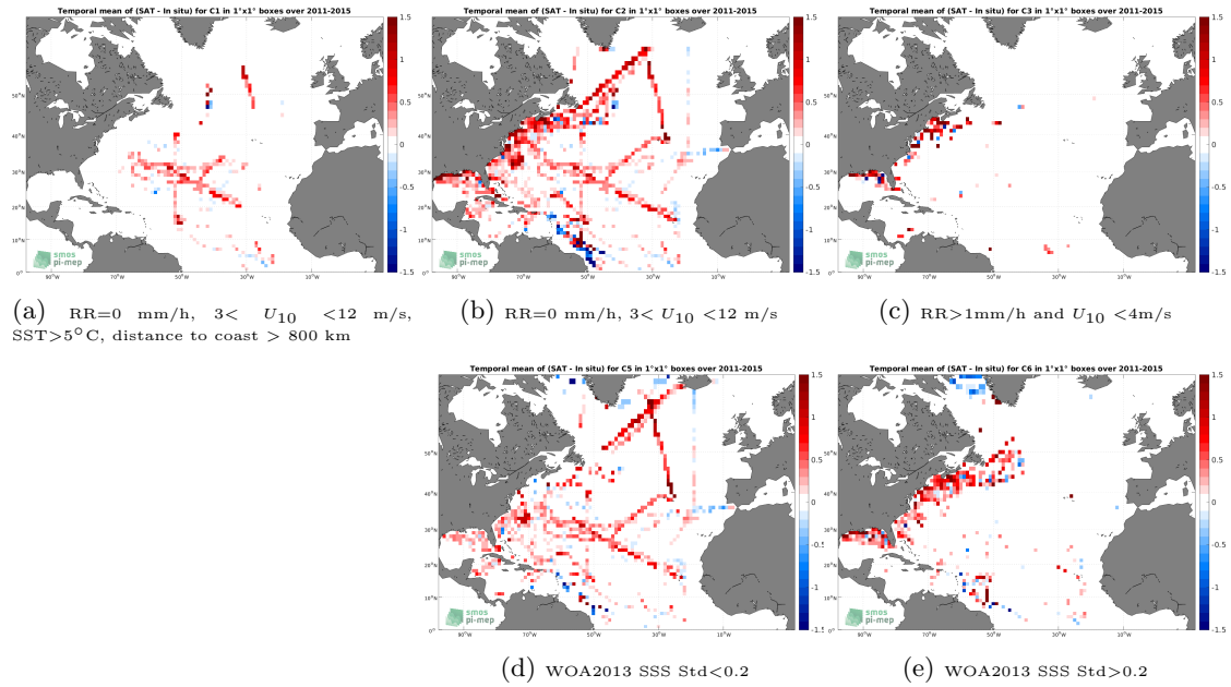
Figure 12: Temporal mean gridded over spatial boxes of size 1^\circ \times 1^\circ of \Delta SSS (Aquarius SSS L3 OR v5 - Monthly - Rain mask (NASA-GSFC) - TSG (SAMOS)) for 5 different subdatasets corresponding to:RR=0 mm/h, 3 < U_{10} < 12 m/s, SST >5^\circ\text{C} , distance to coast > 800 km (a), RR=0 mm/h, 3 < U_{10} < 12 m/s (b), RR >1 mm/h and U_{10} < 4 m/s (c), WOA2013 SSS Std <0.2 (d), WOA2013 SSS Std >0.2 (e).
