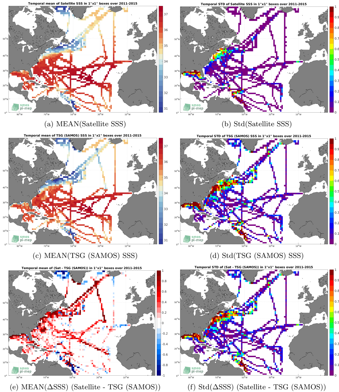
Figure 6: Temporal mean (left) and Std (right) of SSS from Aquarius SSS L3 OR v5 - Monthly - Rain mask (NASA-GSFC) (top), TSG (SAMOS) (middle), and of \Delta SSS (Satellite - TSG (SAMOS)). Only match-up pairs are used to generate these maps.
