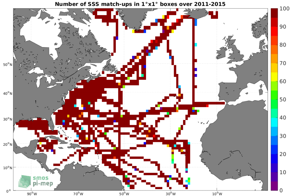
Figure 4: Number of SSS match-ups between TSG (SAMOS) SSS and the Aquarius SSS L3 OR v5 - Monthly - Rain mask (NASA-GSFC) SSS product for the North Atlantic Ocean Pi-MEP region over 1^\circ \times 1^\circ boxes and for the full satellite product period.
