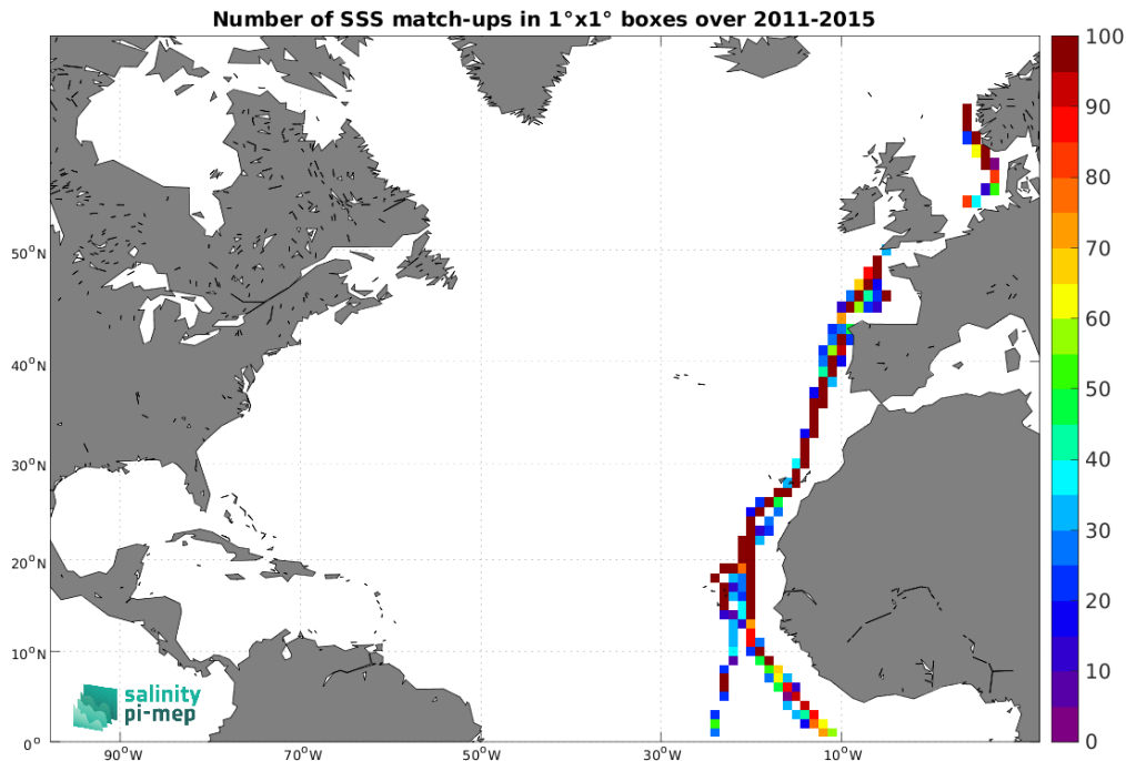
Figure 5: Number of SSS match-ups between TSG (Polarstern) SSS and the Aquarius SSS L3 OR v5 - Monthly - Rain mask (NASA-GSFC) SSS product for the North Atlantic Ocean Pi-MEP region over 1^\circ \times 1^\circ boxes and for the full satellite product period.
