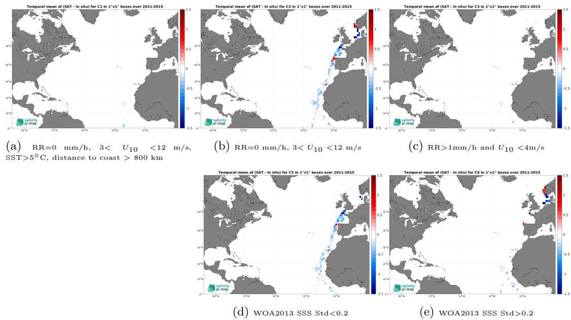
Figure 14: Temporal mean gridded over spatial boxes of size 1^\circ \times 1^\circ of \Delta\text{SSS} (Aquarius SSS L3 OR v5 - Monthly - Rain mask (NASA-GSFC) - TSG (Polarstern)) for 5 different subdatasets corresponding to:RR=0 mm/h, 3 < U_{10} < 12 m/s, SST >5^\circ\text{C} , distance to coast > 800 km (a), RR=0 mm/h, 3 < U_{10} < 12 m/s (b), RR >1 mm/h and U_{10} < 4 m/s (c), WOA2013 SSS Std <0.2 (d), WOA2013 SSS Std >0.2 (e).
