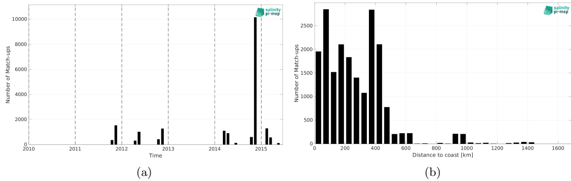
Figure 2: Number of match-ups between TSG (Polarstern) and Aquarius SSS L3 OR v5 - Monthly - Rain mask (NASA-GSFC) SSS as a function of time (a) and as function of the distance to coast (b) over the North Atlantic Ocean Pi-MEP region and for the full satellite product period.
