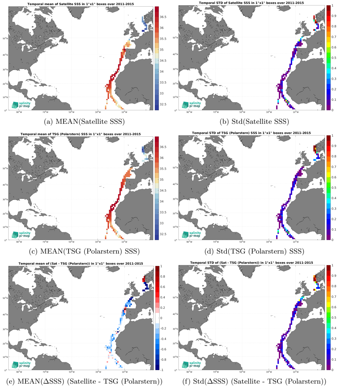
Figure 7: Temporal mean (left) and Std (right) of SSS from Aquarius SSS L3 OR v5 - Monthly - Rain mask (NASA-GSFC) (top), TSG (Polarstern) (middle), and of \Delta SSS (Satellite - TSG (Polarstern)). Only match-up pairs are used to generate these maps.
