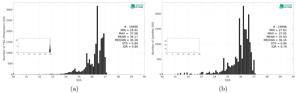
Figure 3: Histograms of SSS from TSG (Polarstern) (a) and Aquarius SSS L3 OR v5 - Monthly - Rain mask (NASA-GSFC) (b) considering all match-up pairs per bins of 0.1 over the North Atlantic Ocean Pi-MEP region and for the full satellite product period.
