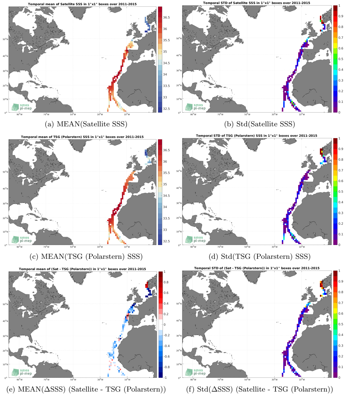
Figure 6: Temporal mean (left) and Std (right) of SSS from Aquarius SSS L3 OR v5 - Monthly - Rain mask (NASA-GSFC) (top), TSG (Polarstern) (middle), and of \Delta SSS (Satellite - TSG (Polarstern)). Only match-up pairs are used to generate these maps.
