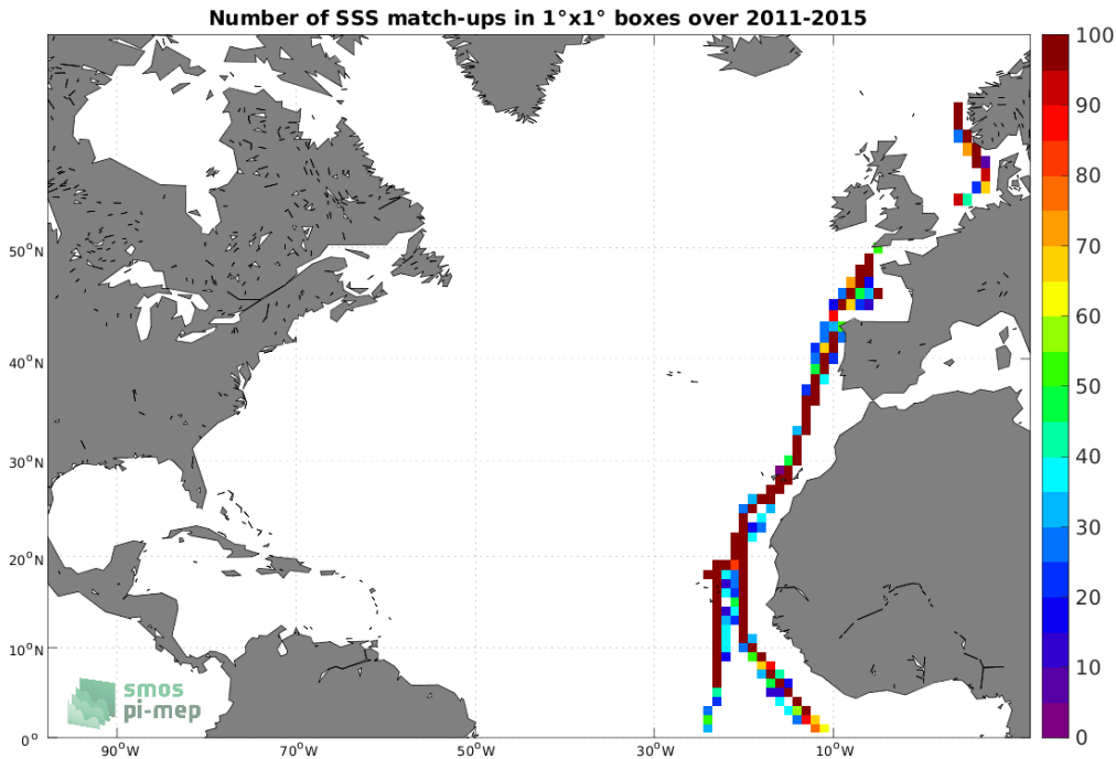
Figure 4: Number of SSS match-ups between TSG (Polarstern) SSS and the Aquarius SSS L3 OR v5 - Monthly - Rain mask (NASA-GSFC) SSS product for the North Atlantic Ocean Pi-MEP region over 1^\circ \times 1^\circ boxes and for the full satellite product period.
