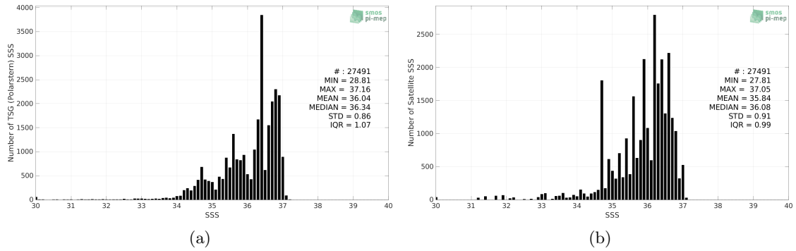
Figure 2: Histograms of SSS from TSG (Polarstern) (a) and Aquarius SSS L3 OR v5 - Monthly - Rain mask (NASA-GSFC) (b) considering all match-up pairs per bins of 0.1 over the North Atlantic Ocean Pi-MEP region and for the full satellite product period.
