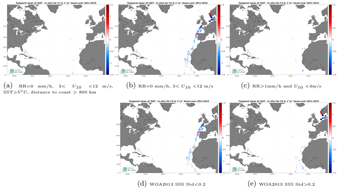
Figure 12: Temporal mean gridded over spatial boxes of size 1^\circ \times 1^\circ of \Delta\text{SSS} (Aquarius SSS L3 OR v5 - Monthly - Rain mask (NASA-GSFC) - TSG (Polarstern)) for 5 different subdatasets corresponding to:RR=0 mm/h, 3 < U_{10} < 12 m/s, SST >5^\circ\text{C} , distance to coast > 800 km (a), RR=0 mm/h, 3 < U_{10} < 12 m/s (b), RR >1 mm/h and U_{10} < 4 m/s (c), WOA2013 SSS Std <0.2 (d), WOA2013 SSS Std >0.2 (e).
