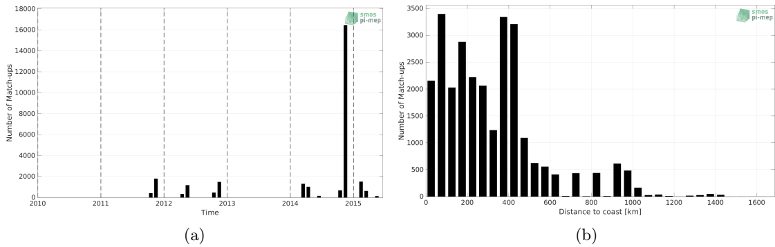
Figure 1: Number of match-ups between TSG (Polarstern) and Aquarius SSS L3 OR v5 - Monthly - Rain mask (NASA-GSFC) SSS as a function of time (a) and as function of the distance to coast (b) over the North Atlantic Ocean Pi-MEP region and for the full satellite product period.
