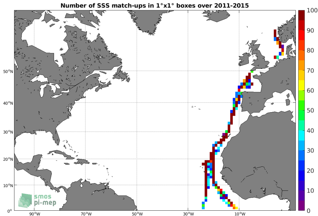
Figure 4: Number of SSS match-ups between TSG (Polarstern) SSS and the Aquarius SSS L3 OR v5 - Monthly - Rain mask (NASA-GSFC) SSS product for the North Atlantic Ocean Pi-MEP region over 1°x1° boxes and for the full satellite product period.
