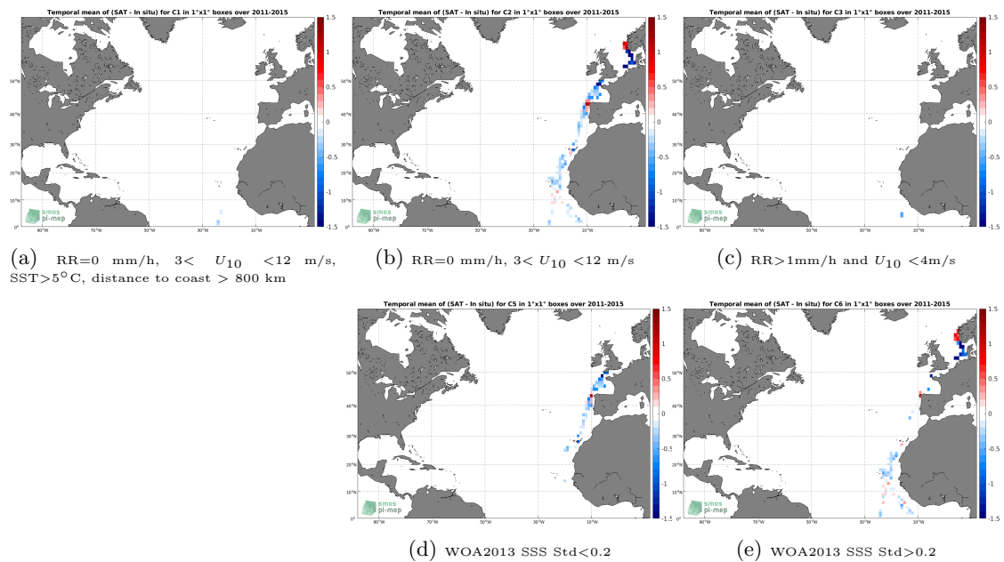
Figure 12: Temporal mean gridded over spatial boxes of size 1^\circ \times 1^\circ of \Delta SSS (Aquarius SSS L3 OR v5 - Monthly - Rain mask (NASA-GSFC) - TSG (Polarstern)) for 5 different subdatasets corresponding to: RR=0 mm/h, 3 < U_{10} < 12 m/s, SST > 5^\circ\text{C} , distance to coast > 800 km (a), RR=0 mm/h, 3 < U_{10} < 12 m/s (b), RR > 1 mm/h and U_{10} < 4 m/s (c), WOA2013 SSS Std < 0.2 (d), WOA2013 SSS Std > 0.2 (e).
