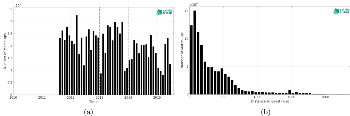
Figure 2: Number of match-ups between TSG (LEGOS-DM) and Aquarius SSS L3 OR v5 - Monthly - Rain mask (NASA-GSFC) SSS as a function of time (a) and as function of the distance to coast (b) over the North Atlantic Ocean Pi-MEP region and for the full satellite product period.
