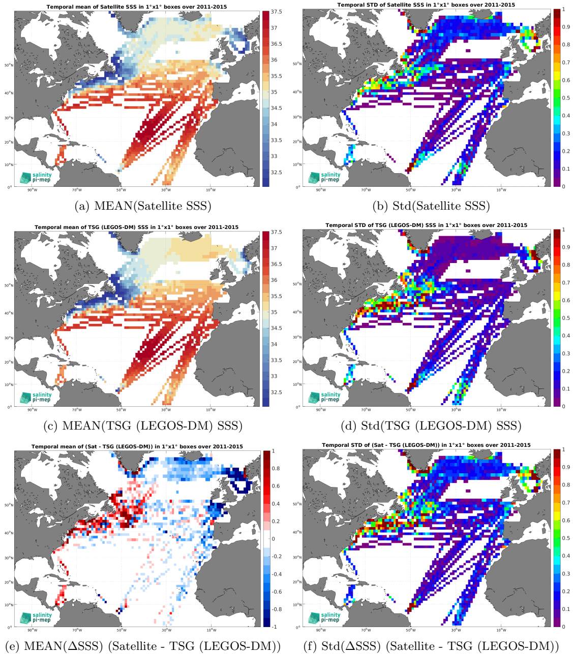
Figure 7: Temporal mean (left) and Std (right) of SSS from Aquarius SSS L3 OR v5 - Monthly - Rain mask (NASA-GSFC) (top), TSG (LEGOS-DM) (middle), and of \Delta SSS (Satellite - TSG (LEGOS-DM)). Only match-up pairs are used to generate these maps.
