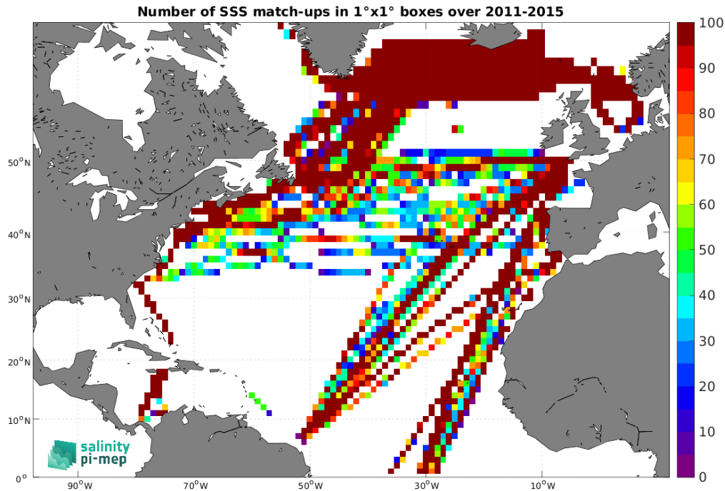
Figure 5: Number of SSS match-ups between TSG (LEGOS-DM) SSS and the Aquarius SSS L3 OR v5 - Monthly - Rain mask (NASA-GSFC) SSS product for the North Atlantic Ocean Pi-MEP region over 1^\circ \times 1^\circ boxes and for the full satellite product period.
