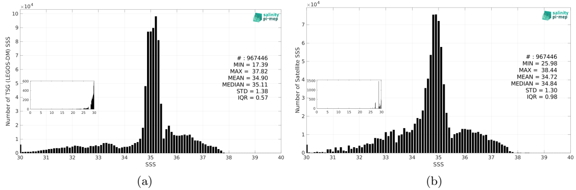
Figure 3: Histograms of SSS from TSG (LEGOS-DM) (a) and Aquarius SSS L3 OR v5 - Monthly - Rain mask (NASA-GSFC) (b) considering all match-up pairs per bins of 0.1 over the North Atlantic Ocean Pi-MEP region and for the full satellite product period.
