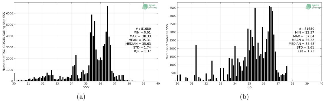
Figure 2: Histograms of SSS from TSG-GOSUD-Sailing-ship (a) and Aquarius-L3-OR-V5-MONTHLY-RAIN-MASK-1DEG (b) considering all match-up pairs per bins of 0.1 over the North Atlantic Ocean Pi-MEP region and for the full satellite product period.
