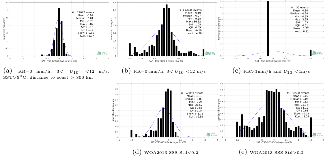
Figure 13: Normalized histogram of \Delta SSS (Aquarius-L3-OR-V5-MONTHLY-RAIN-MASK-1DEG - TSG-GOSUD-Sailing-ship) for 5 different subdatasets corresponding to: RR=0 mm/h, 3 < U_{10} < 12 m/s, SST>5°C, distance to coast > 800 km (a), RR=0 mm/h, 3 < U_{10} < 12 m/s (b), RR>1mm/h and U_{10} < 4 m/s (c), WOA2013 SSS Std<0.2 (d), WOA2013 SSS Std>0.2 (e).
