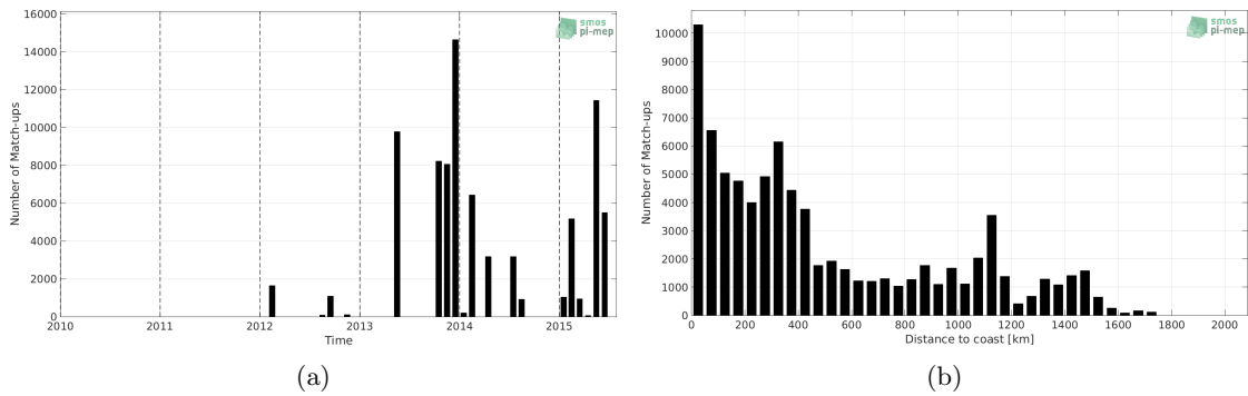
Figure 1: Number of match-ups between TSG-GOSUD-Sailing-ship and Aquarius-L3-OR-V5-MONTHLY-RAIN-MASK-1DEG SSS as a function of time (a) and as function of the distance to coast (b) over the North Atlantic Ocean Pi-MEP region and for the full satellite product period.
