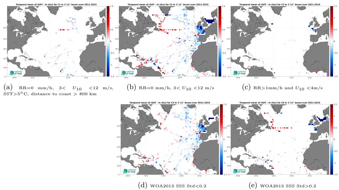
Figure 14: Temporal mean gridded over spatial boxes of size 1^\circ \times 1^\circ of \Delta\text{SSS} (Aquarius SSS L3 OR v5 - Monthly - Rain mask (NASA-GSFC) - TSG (GOSUD-Research-vessel)) for 5 different subdatasets corresponding to:RR=0 mm/h, 3 < U_{10} < 12 m/s, SST >5^\circ\text{C} , distance to coast > 800 km (a), RR=0 mm/h, 3 < U_{10} < 12 m/s (b), RR >1 mm/h and U_{10} < 4 m/s (c), WOA2013 SSS Std <0.2 (d), WOA2013 SSS Std >0.2 (e).
