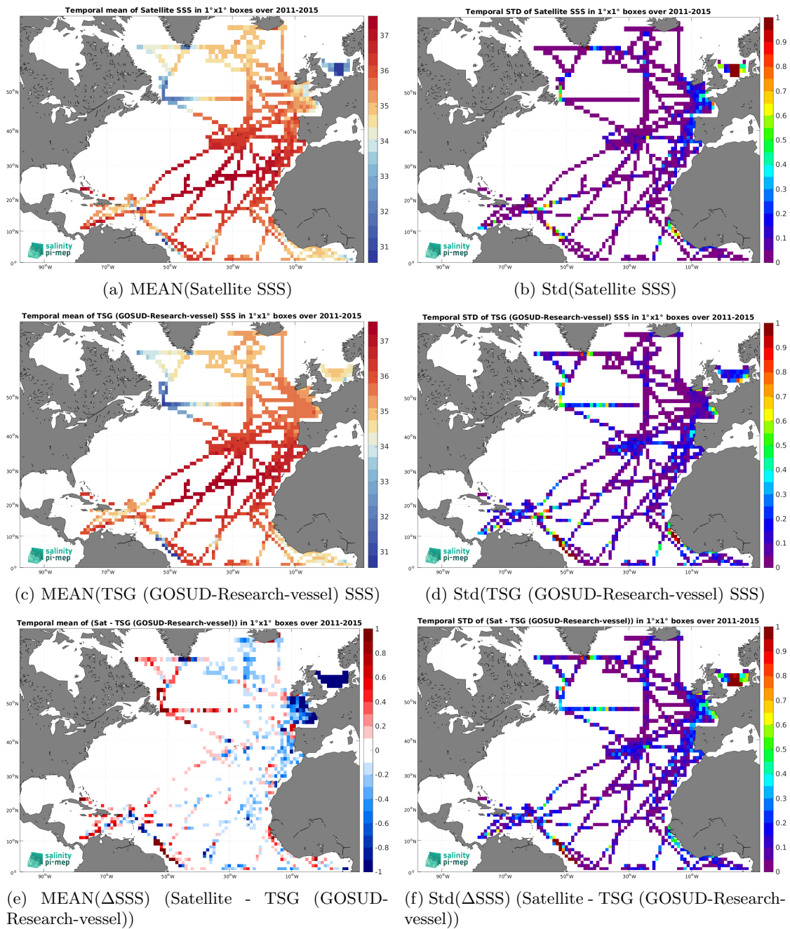
Figure 7: Temporal mean (left) and Std (right) of SSS from Aquarius SSS L3 OR v5 - Monthly - Rain mask (NASA-GSFC) (top), TSG (GOSUD-Research-vessel) (middle), and of \Delta SSS (Satellite - TSG (GOSUD-Research-vessel)). Only match-up pairs are used to generate these maps.
