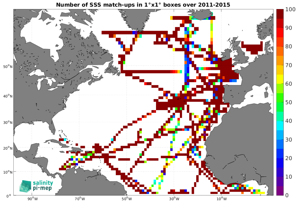
Figure 5: Number of SSS match-ups between TSG (GOSUD-Research-vessel) SSS and the Aquarius SSS L3 OR v5 - Monthly - Rain mask (NASA-GSFC) SSS product for the North Atlantic Ocean Pi-MEP region over 1^\circ \times 1^\circ boxes and for the full satellite product period.
