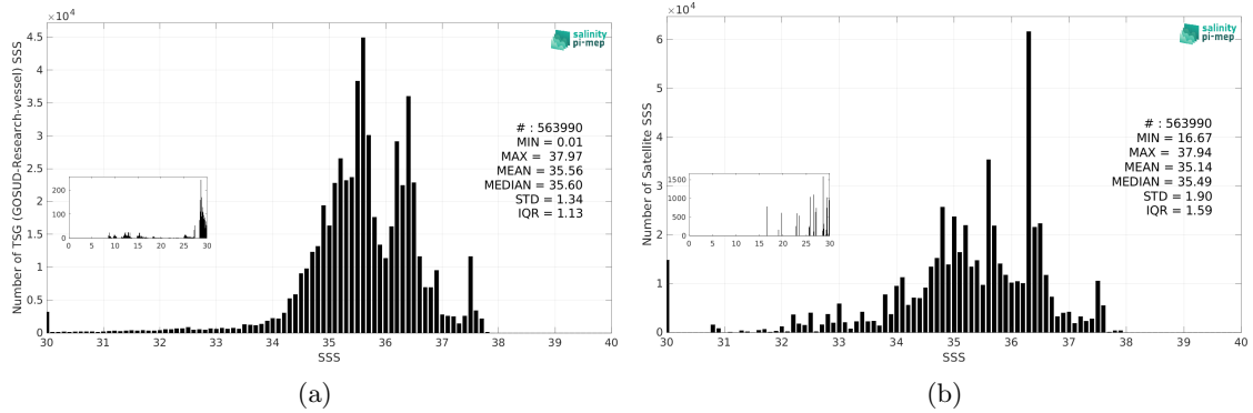
Figure 3: Histograms of SSS from TSG (GOSUD-Research-vessel) (a) and Aquarius SSS L3 OR v5 - Monthly - Rain mask (NASA-GSFC) (b) considering all match-up pairs per bins of 0.1 over the North Atlantic Ocean Pi-MEP region and for the full satellite product period.
