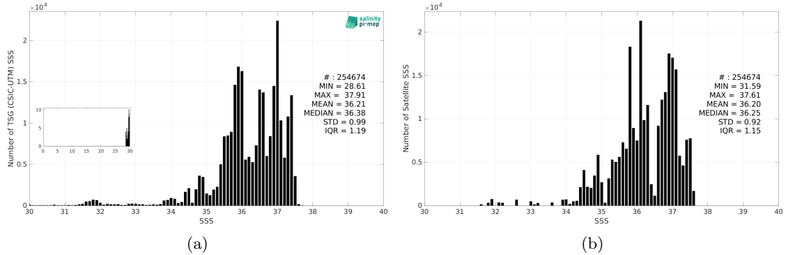
Figure 3: Histograms of SSS from TSG (CSIC-UTM) (a) and Aquarius SSS L3 OR v5 - Monthly - Rain mask (NASA-GSFC) (b) considering all match-up pairs per bins of 0.1 over the North Atlantic Ocean Pi-MEP region and for the full satellite product period.
