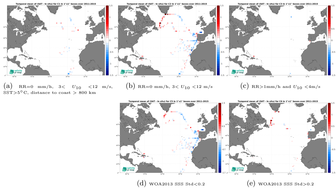
Figure 14: Temporal mean gridded over spatial boxes of size 1^\circ \times 1^\circ of \Delta SSS (Aquarius SSS L3 OR v5 - Monthly - Rain mask (NASA-GSFC) - TSG (CSIC-UTM)) for 5 different subdatasets corresponding to:RR=0 mm/h, 3 < U_{10} < 12 m/s, SST >5^\circ\text{C} , distance to coast > 800 km (a), RR=0 mm/h, 3 < U_{10} < 12 m/s (b), RR >1 mm/h and U_{10} < 4 m/s (c), WOA2013 SSS Std <0.2 (d), WOA2013 SSS Std >0.2 (e).
