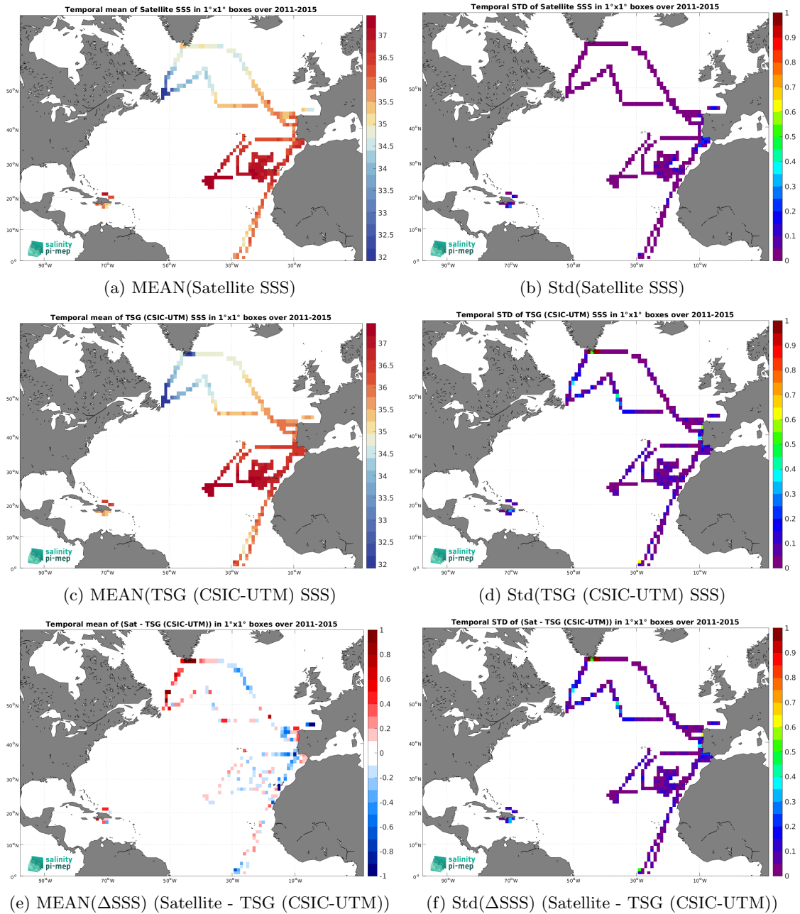
Figure 7: Temporal mean (left) and Std (right) of SSS from Aquarius SSS L3 OR v5 - Monthly - Rain mask (NASA-GSFC) (top), TSG (CSIC-UTM) (middle), and of \Delta SSS (Satellite - TSG (CSIC-UTM)). Only match-up pairs are used to generate these maps.
