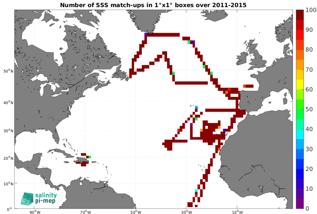
Figure 5: Number of SSS match-ups between TSG (CSIC-UTM) SSS and the Aquarius SSS L3 OR v5 - Monthly - Rain mask (NASA-GSFC) SSS product for the North Atlantic Ocean Pi-MEP region over 1^\circ \times 1^\circ boxes and for the full satellite product period.
