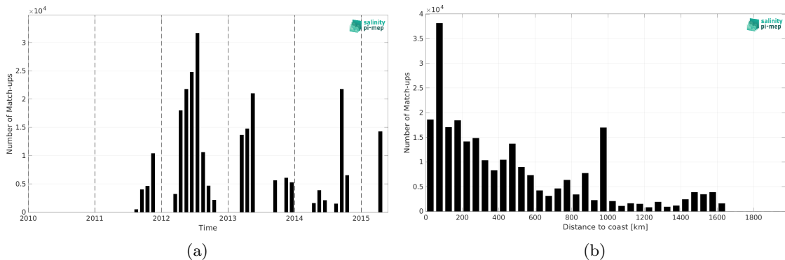
Figure 2: Number of match-ups between TSG (CSIC-UTM) and Aquarius SSS L3 OR v5 - Monthly - Rain mask (NASA-GSFC) SSS as a function of time (a) and as function of the distance to coast (b) over the North Atlantic Ocean Pi-MEP region and for the full satellite product period.
