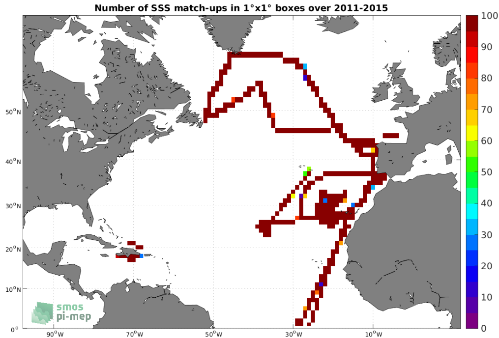
Figure 4: Number of SSS match-ups between TSG (CSIC-UTM) SSS and the Aquarius SSS L3 OR v5 - Monthly - Rain mask (NASA-GSFC) SSS product for the North Atlantic Ocean Pi-MEP region over 1^\circ \times 1^\circ boxes and for the full satellite product period.
