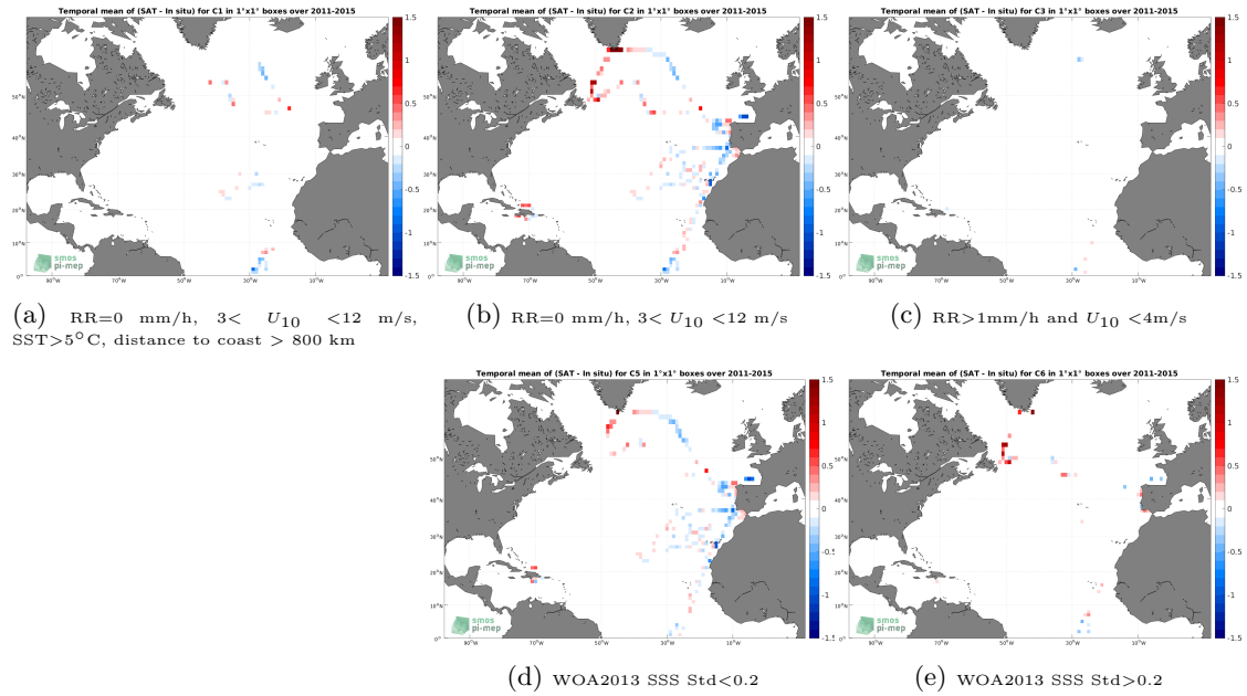
Figure 12: Temporal mean gridded over spatial boxes of size 1^\circ \times 1^\circ of \Delta SSS (Aquarius SSS L3 OR v5 - Monthly - Rain mask (NASA-GSFC) - TSG (CSIC-UTM)) for 5 different subdatasets corresponding to:RR=0 mm/h, 3 < U_{10} < 12 m/s, SST >5^\circ\text{C} , distance to coast > 800 km (a), RR=0 mm/h, 3 < U_{10} < 12 m/s (b), RR >1 mm/h and U_{10} < 4 m/s (c), WOA2013 SSS Std <0.2 (d), WOA2013 SSS Std >0.2 (e).
