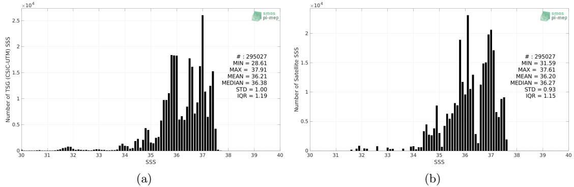
Figure 2: Histograms of SSS from TSG (CSIC-UTM) (a) and Aquarius SSS L3 OR v5 - Monthly - Rain mask (NASA-GSFC) (b) considering all match-up pairs per bins of 0.1 over the North Atlantic Ocean Pi-MEP region and for the full satellite product period.
