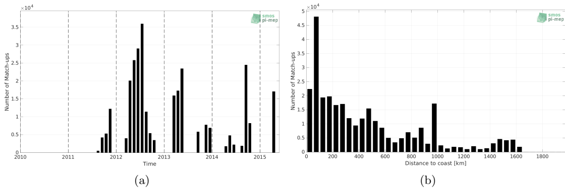
Figure 1: Number of match-ups between TSG (CSIC-UTM) and Aquarius SSS L3 OR v5 - Monthly - Rain mask (NASA-GSFC) SSS as a function of time (a) and as function of the distance to coast (b) over the North Atlantic Ocean Pi-MEP region and for the full satellite product period.
