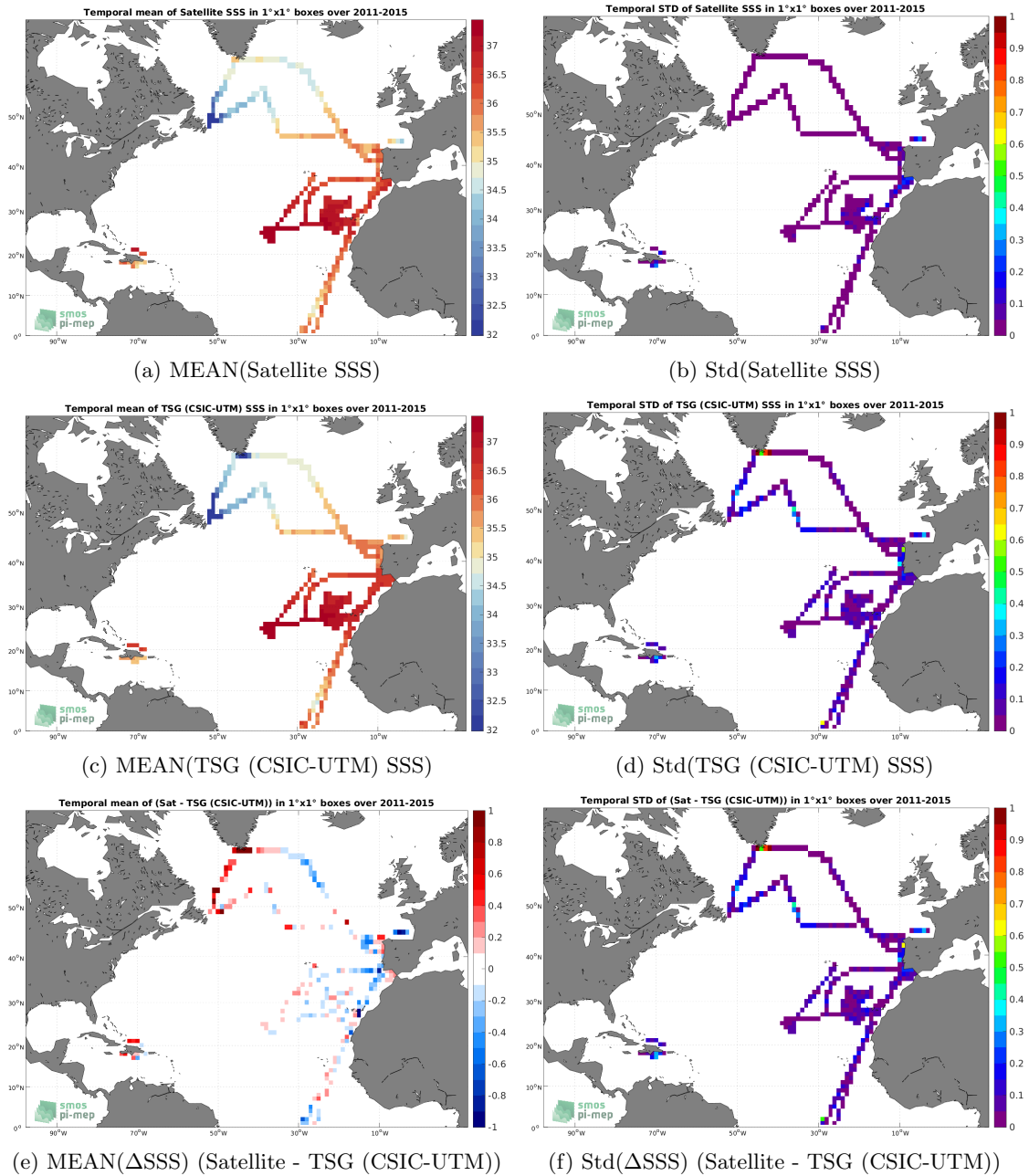
Figure 6: Temporal mean (left) and Std (right) of SSS from Aquarius SSS L3 OR v5 - Monthly - Rain mask (NASA-GSFC) (top), TSG (CSIC-UTM) (middle), and of \Delta SSS (Satellite - TSG (CSIC-UTM)). Only match-up pairs are used to generate these maps.
