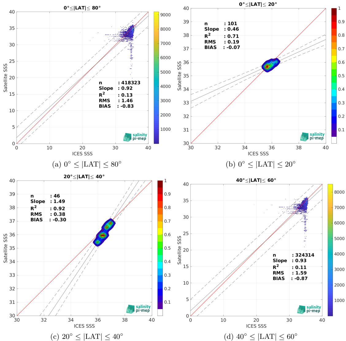
Figure 10: Contour maps of the concentration of Aquarius SSS L3 OR v5 - Monthly - Rain mask (NASA-GSFC) SSS (y-axis) versus ICES SSS (x-axis) at match-up pairs for different latitude bands. For each plot, the red line shows x=y . The black thin and dashed lines indicate a linear fit through the data cloud and the \pm 95\% confidence levels, respectively. The number match-up pairs n , the slope and R^2 coefficient of the linear fit, the root mean square (RMS) and the mean bias between satellite and in situ data are indicated for each latitude band in each plots.
