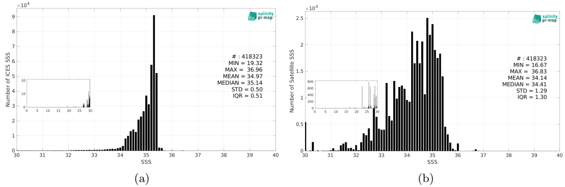
Figure 3: Histograms of SSS from ICES (a) and Aquarius SSS L3 OR v5 - Monthly - Rain mask (NASA-GSFC) (b) considering all match-up pairs per bins of 0.1 over the North Atlantic Ocean Pi-MEP region and for the full satellite product period.
