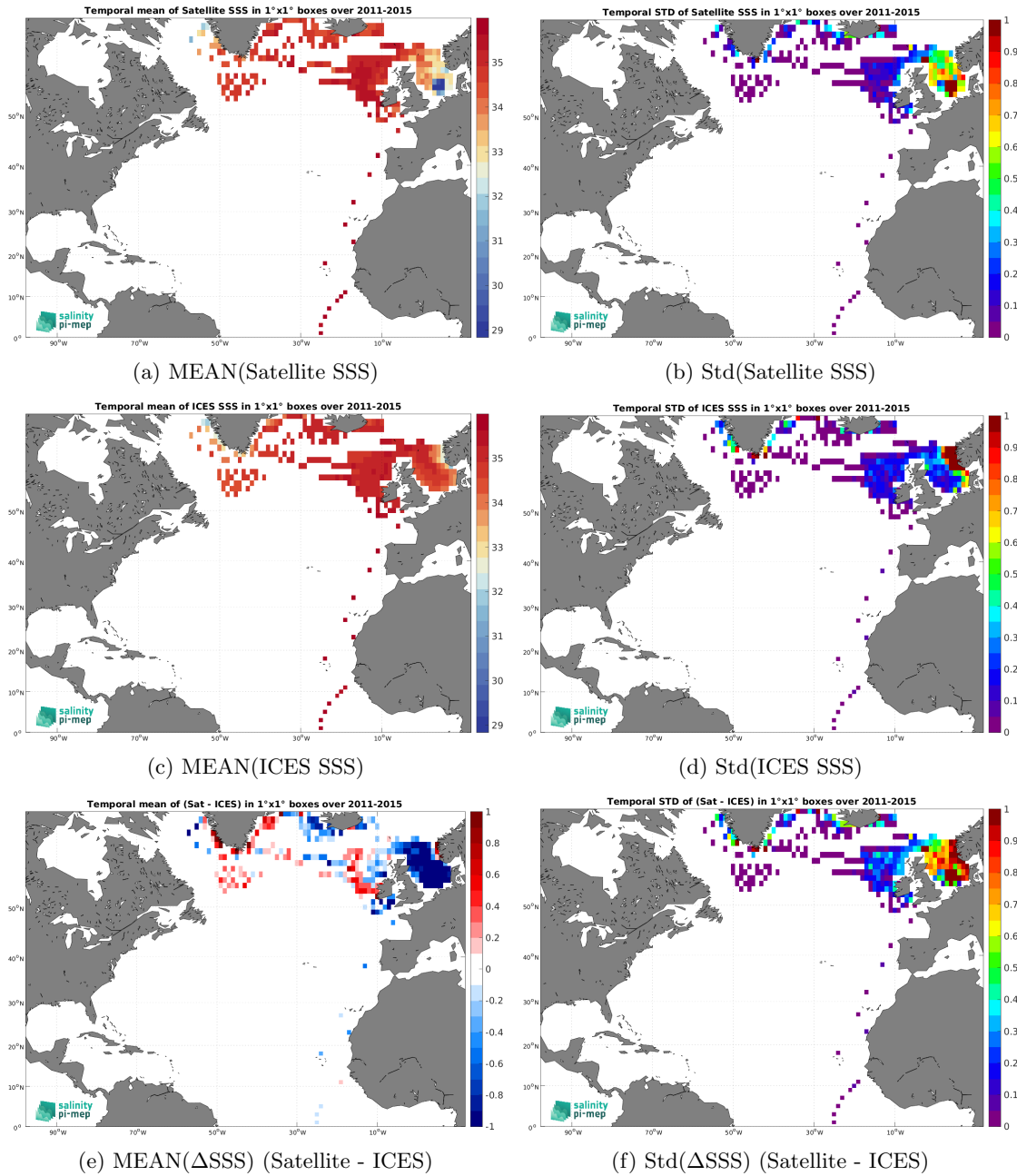
Figure 7: Temporal mean (left) and Std (right) of SSS from Aquarius SSS L3 OR v5 - Monthly - Rain mask (NASA-GSFC) (top), ICES (middle), and of \Delta SSS (Satellite - ICES). Only match-up pairs are used to generate these maps.
