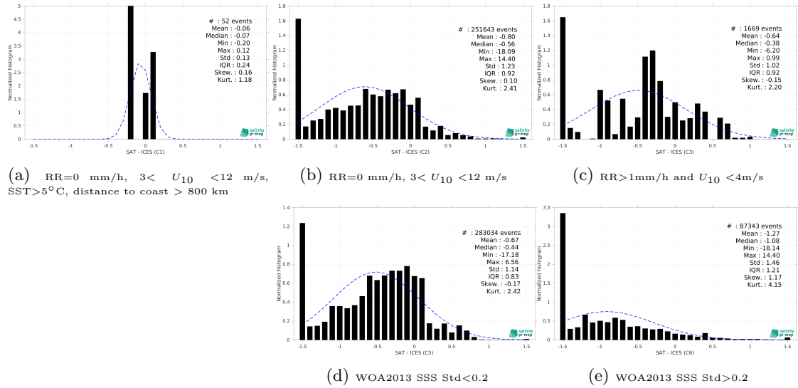
Figure 15: Normalized histogram of \Delta SSS (Aquarius SSS L3 OR v5 - Monthly - Rain mask (NASA-GSFC) - ICES) for 5 different subdatasets corresponding to: RR=0 mm/h, 3 < U_{10} < 12 m/s, SST > 5°C, distance to coast > 800 km (a), RR=0 mm/h, 3 < U_{10} < 12 m/s (b), RR > 1mm/h and U_{10} < 4 m/s (c), WOA2013 SSS Std < 0.2 (d), WOA2013 SSS Std > 0.2 (e).
