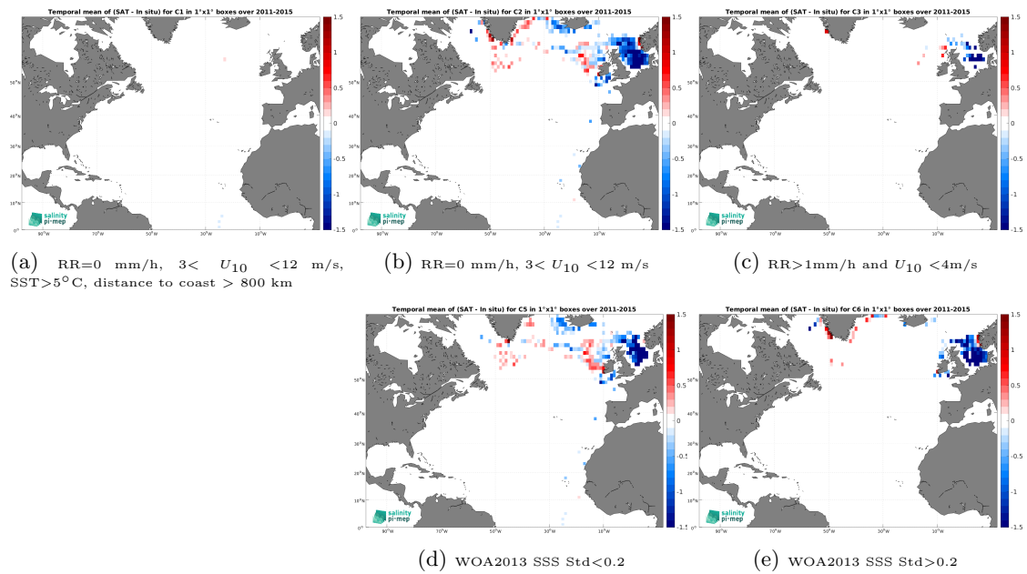
Figure 14: Temporal mean gridded over spatial boxes of size 1^\circ \times 1^\circ of \Delta\text{SSS} (Aquarius SSS L3 OR v5 - Monthly - Rain mask (NASA-GSFC) - ICES) for 5 different subdatasets corresponding to:RR=0 mm/h, 3 < U_{10} < 12 m/s, SST >5^\circ\text{C} , distance to coast > 800 km (a), RR=0 mm/h, 3 < U_{10} < 12 m/s (b), RR >1 mm/h and U_{10} < 4 m/s (c), WOA2013 SSS Std <0.2 (d), WOA2013 SSS Std >0.2 (e).
