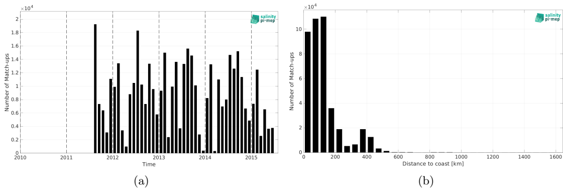
Figure 2: Number of match-ups between ICES and Aquarius SSS L3 OR v5 - Monthly - Rain mask (NASA-GSFC) SSS as a function of time (a) and as function of the distance to coast (b) over the North Atlantic Ocean Pi-MEP region and for the full satellite product period.
