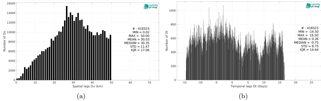
Figure 6: Histograms of the spatial (a) and temporal (b) lags between the location/time of the ICES measurement and the date of the corresponding Aquarius SSS L3 OR v5 - Monthly - Rain mask (NASA-GSFC) SSS pixel.
