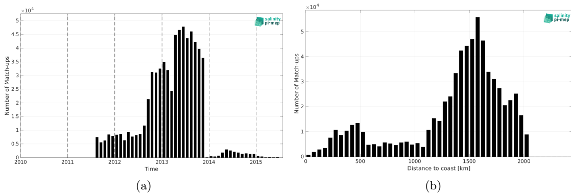
Figure 2: Number of match-ups between Surface drifters and Aquarius SSS L3 OR v5 - Monthly - Rain mask (NASA-GSFC) SSS as a function of time (a) and as function of the distance to coast (b) over the North Atlantic Ocean Pi-MEP region and for the full satellite product period.
