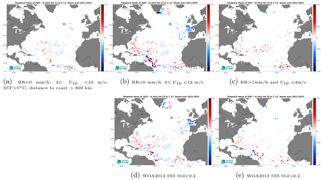
Figure 13: Temporal mean gridded over spatial boxes of size 1^\circ \times 1^\circ of \Delta\text{SSS} (Aquarius SSS L3 OR v5 - Monthly - Rain mask (NASA-GSFC) - Surface drifters) for 5 different subdatasets corresponding to:RR=0 mm/h, 3 < U_{10} < 12 m/s, SST >5^\circ\text{C} , distance to coast > 800 km (a), RR=0 mm/h, 3 < U_{10} < 12 m/s (b), RR >1 mm/h and U_{10} < 4 m/s (c), WOA2013 SSS Std <0.2 (d), WOA2013 SSS Std >0.2 (e).
