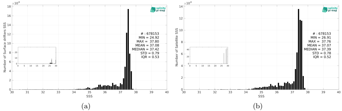
Figure 3: Histograms of SSS from Surface drifters (a) and Aquarius SSS L3 OR v5 - Monthly - Rain mask (NASA-GSFC) (b) considering all match-up pairs per bins of 0.1 over the North Atlantic Ocean Pi-MEP region and for the full satellite product period.
