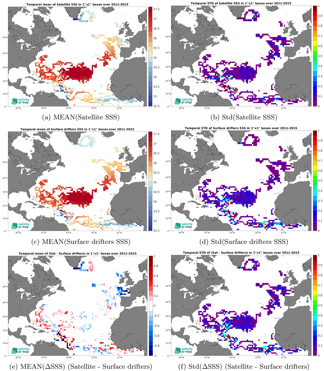
Figure 6: Temporal mean (left) and Std (right) of SSS from Aquarius SSS L3 OR v5 - Monthly - Rain mask (NASA-GSFC) (top), Surface drifters (middle), and of \Delta SSS (Satellite - Surface drifters). Only match-up pairs are used to generate these maps.
