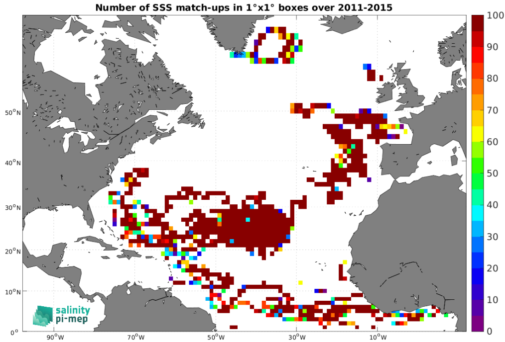
Figure 4: Number of SSS match-ups between Surface drifters SSS and the Aquarius SSS L3 OR v5 - Monthly - Rain mask (NASA-GSFC) SSS product for the North Atlantic Ocean Pi-MEP region over 1^\circ \times 1^\circ boxes and for the full satellite product period.
