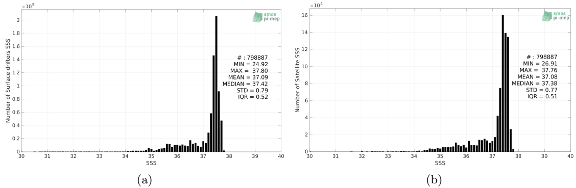
Figure 2: Histograms of SSS from Surface drifters (a) and Aquarius SSS L3 OR v5 - Monthly - Rain mask (NASA-GSFC) (b) considering all match-up pairs per bins of 0.1 over the North Atlantic Ocean Pi-MEP region and for the full satellite product period.
