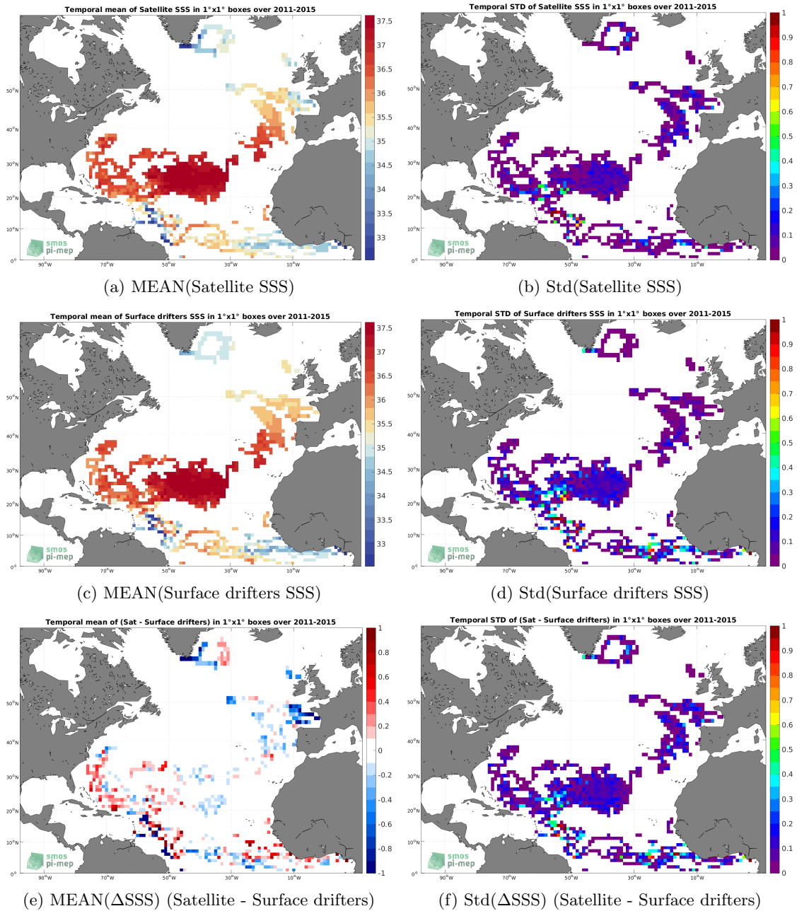
Figure 5: Temporal mean (left) and Std (right) of SSS from Aquarius SSS L3 OR v5 - Monthly - Rain mask (NASA-GSFC) (top), Surface drifters (middle), and of \Delta SSS (Satellite - Surface drifters). Only match-up pairs are used to generate these maps.
