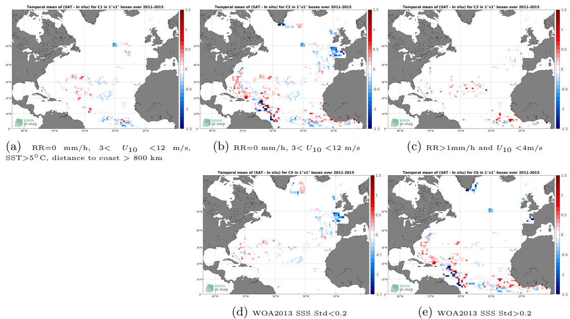
Figure 11: Temporal mean gridded over spatial boxes of size 1^\circ \times 1^\circ of \Delta SSS (Aquarius SSS L3 OR v5 - Monthly - Rain mask (NASA-GSFC) - Surface drifters) for 5 different subdatasets corresponding to:RR=0 mm/h, 3 < U_{10} < 12 m/s, SST >5^\circ\text{C} , distance to coast > 800 km (a), RR=0 mm/h, 3 < U_{10} < 12 m/s (b), RR >1 mm/h and U_{10} < 4 m/s (c), WOA2013 SSS Std <0.2 (d), WOA2013 SSS Std >0.2 (e).
