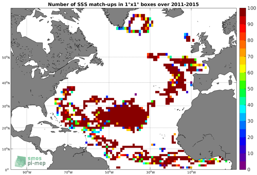
Figure 3: Number of SSS match-ups between Surface drifters SSS and the Aquarius-L3-OR-V5-MONTHLY-RAIN-MASK-1DEG SSS product for the North Atlantic Ocean Pi-MEP region over 1^\circ \times 1^\circ boxes and for the full satellite product period.
