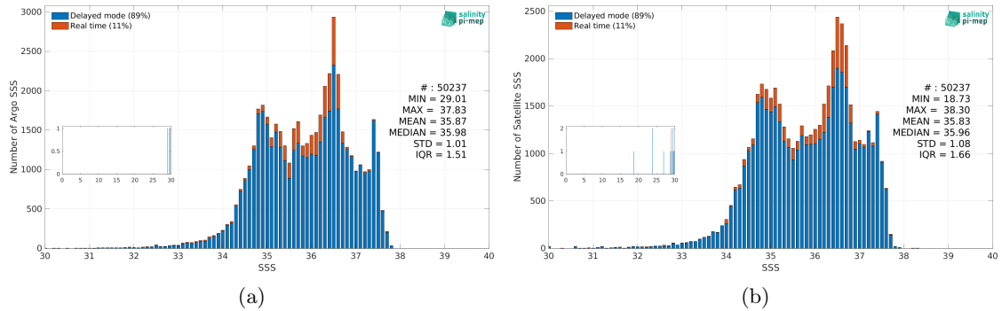
Figure 3: Histograms of SSS from Argo (a) and Aquarius SSS L3 OR v5 - Monthly - Rain mask (NASA-GSFC) (b) considering all match-up pairs per bins of 0.1 over the North Atlantic Ocean Pi-MEP region and for the full satellite product period.
