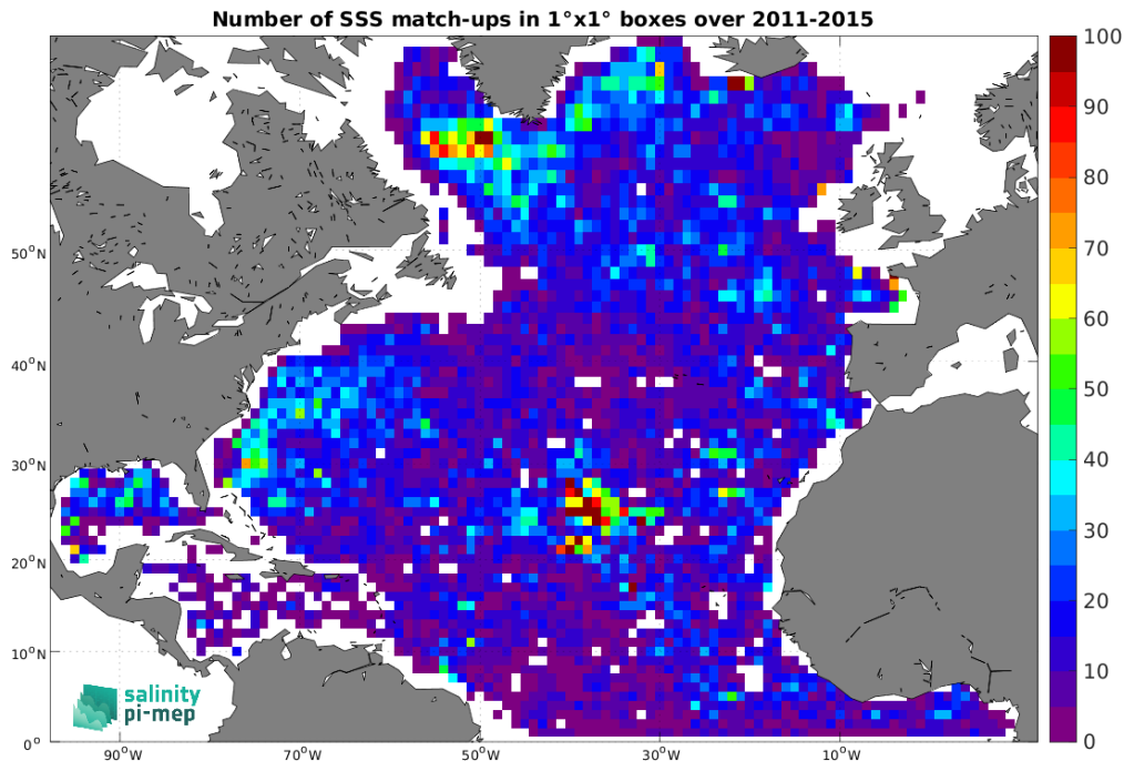
Figure 5: Number of SSS match-ups between Argo SSS and the Aquarius SSS L3 OR v5 - Monthly - Rain mask (NASA-GSFC) SSS product for the North Atlantic Ocean Pi-MEP region over 1^\circ \times 1^\circ boxes and for the full satellite product period.
