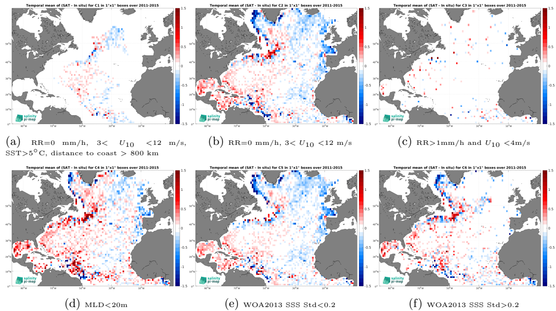
Figure 14: Temporal mean gridded over spatial boxes of size 1^\circ \times 1^\circ of \Delta\text{SSS} (Aquarius SSS L3 OR v5 - Monthly - Rain mask (NASA-GSFC) - Argo) for 6 different subdatasets corresponding to: RR=0 mm/h, 3 < U_{10} < 12 m/s, SST > 5°C, distance to coast > 800 km (a), RR=0 mm/h, 3 < U_{10} < 12 m/s (b), RR > 1mm/h and U_{10} < 4 m/s (c),MLD < 20m (d),WOA2013 SSS Std < 0.2 (e),WOA2013 SSS Std > 0.2 (f).
