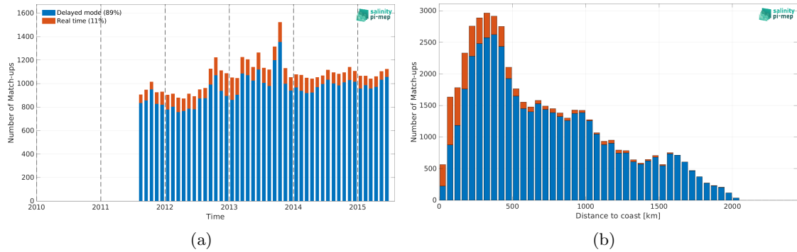
Figure 2: Number of match-ups between Argo and Aquarius SSS L3 OR v5 - Monthly - Rain mask (NASA-GSFC) SSS as a function of time (a) and as function of the distance to coast (b) over the North Atlantic Ocean Pi-MEP region and for the full satellite product period.
