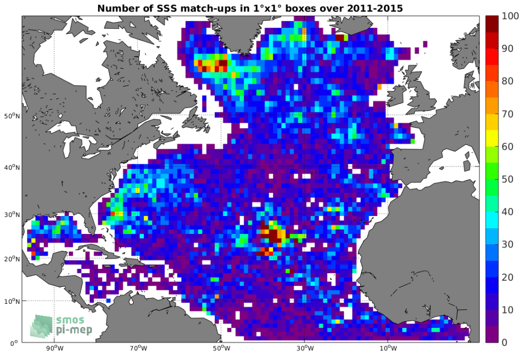
Figure 4: Number of SSS match-ups between Argo SSS and the Aquarius-L3-OR-V5-MONTHLY-RAIN-MASK-1DEG SSS product for the North Atlantic Ocean Pi-MEP region over 1°x1° boxes and for the full satellite product period.
