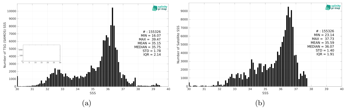
Figure 2: Histograms of SSS from TSG (SAMOS) (a) and Aquarius SSS L3 CAP v5 - 7-Day running (JPL) (b) considering all match-up pairs per bins of 0.1 over the North Atlantic Ocean Pi-MEP region and for the full satellite product period.
