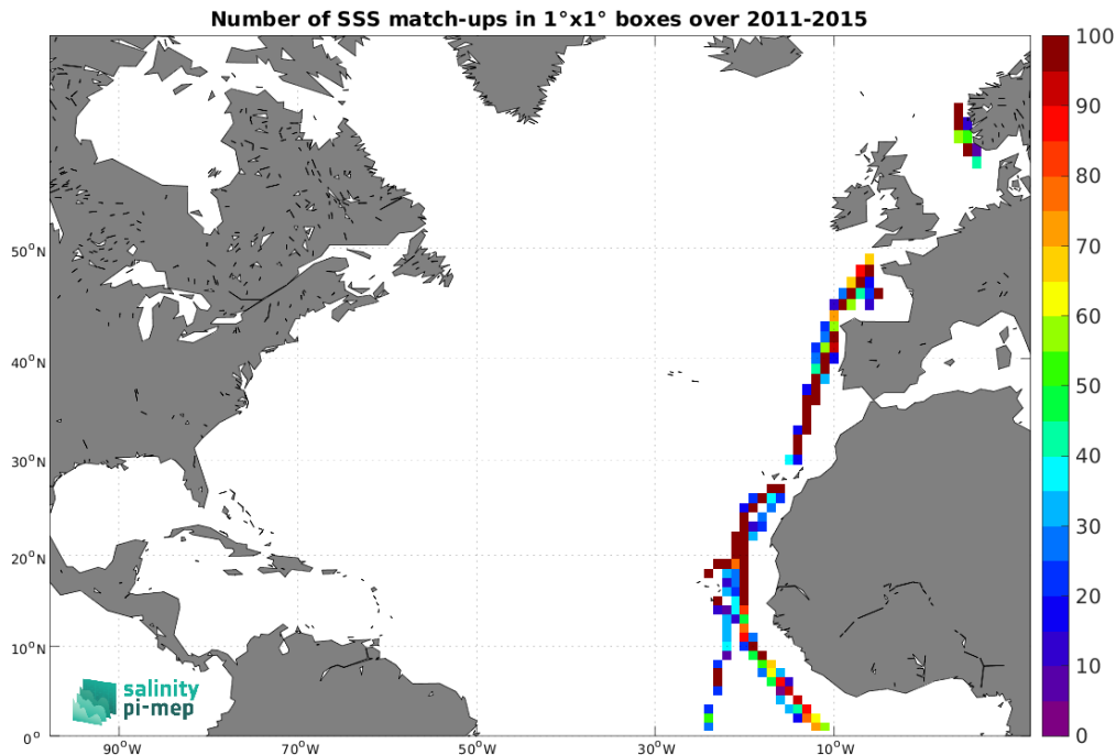
Figure 5: Number of SSS match-ups between TSG (Polarstern) SSS and the Aquarius SSS L3 CAP v5 - 7-Day running (JPL) SSS product for the North Atlantic Ocean Pi-MEP region over 1^\circ \times 1^\circ boxes and for the full satellite product period.
