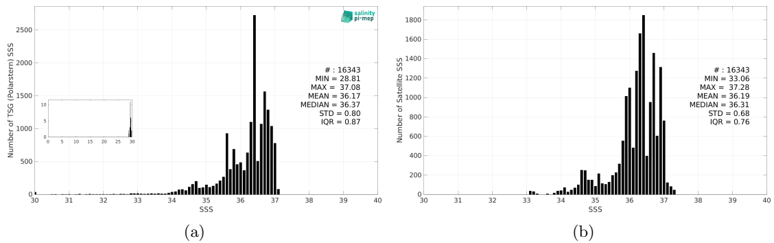
Figure 3: Histograms of SSS from TSG (Polarstern) (a) and Aquarius SSS L3 CAP v5 - 7-Day running (JPL) (b) considering all match-up pairs per bins of 0.1 over the North Atlantic Ocean Pi-MEP region and for the full satellite product period.
