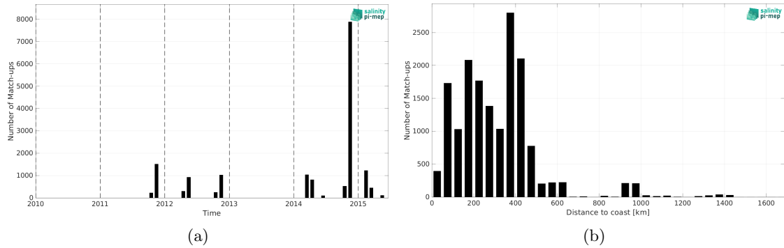
Figure 2: Number of match-ups between TSG (Polarstern) and Aquarius SSS L3 CAP v5 - 7-Day running (JPL) SSS as a function of time (a) and as function of the distance to coast (b) over the North Atlantic Ocean Pi-MEP region and for the full satellite product period.
