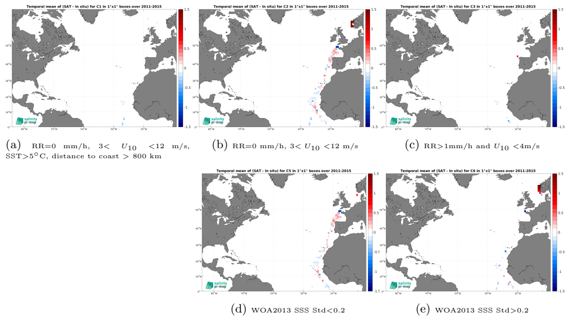
Figure 14: Temporal mean gridded over spatial boxes of size 1^\circ \times 1^\circ of \Delta\text{SSS} (Aquarius SSS L3 CAP v5 - 7-Day running (JPL) - TSG (Polarstern)) for 5 different subdatasets corresponding to:RR=0 mm/h, 3 < U_{10} < 12 m/s, SST>5°C, distance to coast > 800 km (a), RR=0 mm/h, 3 < U_{10} < 12 m/s (b), RR>1mm/h and U_{10} < 4 m/s (c), WOA2013 SSS Std<0.2 (d), WOA2013 SSS Std>0.2 (e).
