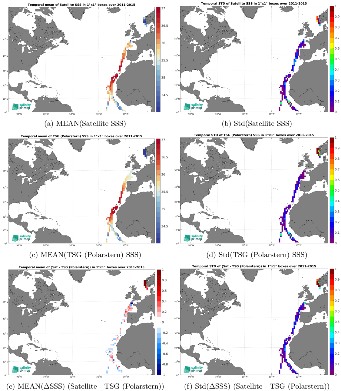
Figure 7: Temporal mean (left) and Std (right) of SSS from Aquarius SSS L3 CAP v5 - 7-Day running (JPL) (top), TSG (Polarstern) (middle), and of \Delta SSS (Satellite - TSG (Polarstern)). Only match-up pairs are used to generate these maps.
