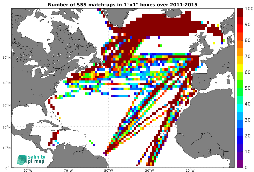
Figure 5: Number of SSS match-ups between TSG (LEGOS-DM) SSS and the Aquarius SSS L3 CAP v5 - 7-Day running (JPL) SSS product for the North Atlantic Ocean Pi-MEP region over 1^\circ \times 1^\circ boxes and for the full satellite product period.
