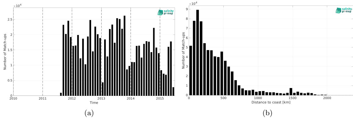
Figure 2: Number of match-ups between TSG (LEGOS-DM) and Aquarius SSS L3 CAP v5 - 7-Day running (JPL) SSS as a function of time (a) and as function of the distance to coast (b) over the North Atlantic Ocean Pi-MEP region and for the full satellite product period.
