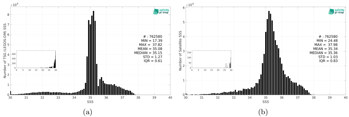
Figure 3: Histograms of SSS from TSG (LEGOS-DM) (a) and Aquarius SSS L3 CAP v5 - 7-Day running (JPL) (b) considering all match-up pairs per bins of 0.1 over the North Atlantic Ocean Pi-MEP region and for the full satellite product period.
