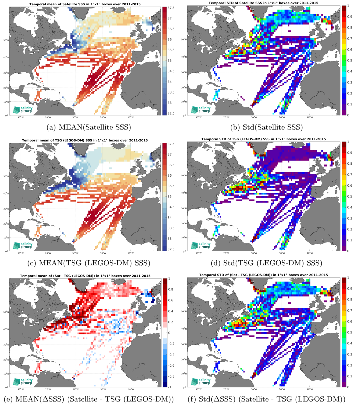
Figure 7: Temporal mean (left) and Std (right) of SSS from Aquarius SSS L3 CAP v5 - 7-Day running (JPL) (top), TSG (LEGOS-DM) (middle), and of \Delta SSS (Satellite - TSG (LEGOS-DM)). Only match-up pairs are used to generate these maps.
