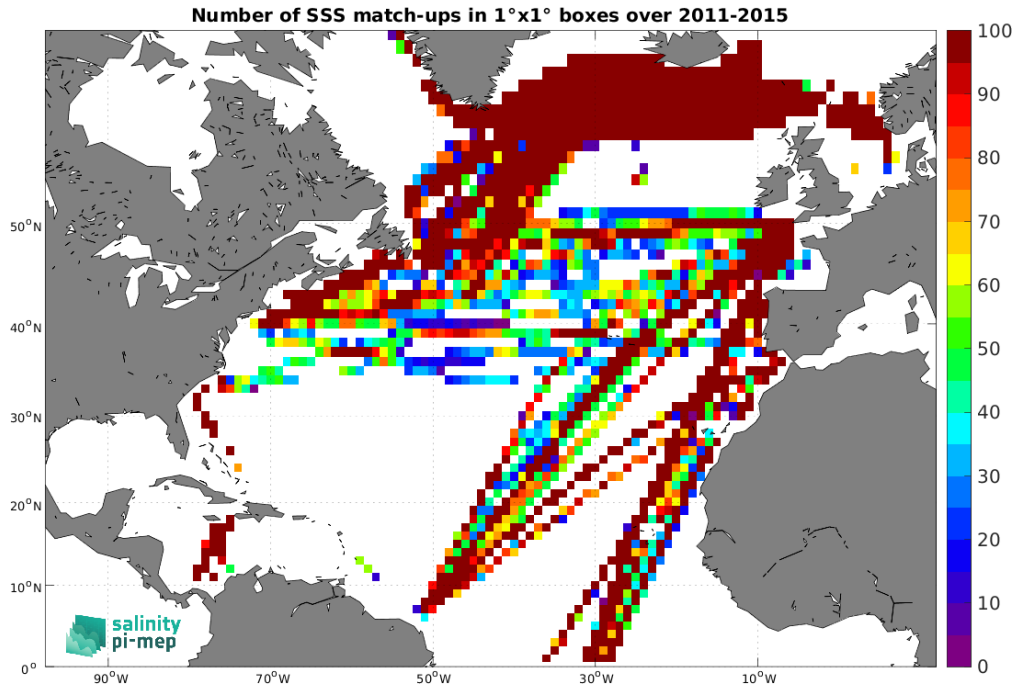
Figure 4: Number of SSS match-ups between TSG (LEGOS-DM) SSS and the Aquarius SSS L3 CAP v5 - 7-Day running (JPL) SSS product for the North Atlantic Ocean Pi-MEP region over 1°×1° boxes and for the full satellite product period.
