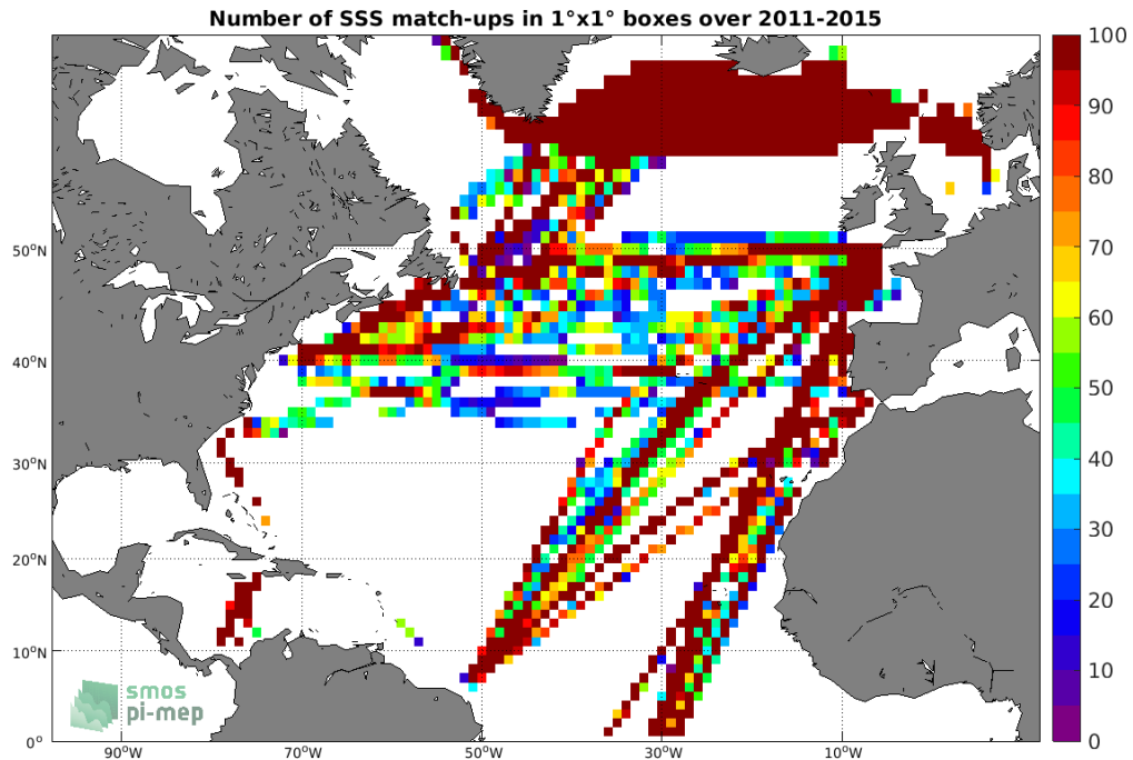
Figure 4: Number of SSS match-ups between TSG (LEGOS-DM) SSS and the Aquarius SSS L3 CAP v5 - 7-Day running (JPL) SSS product for the North Atlantic Ocean Pi-MEP region over 1°x1° boxes and for the full satellite product period.
