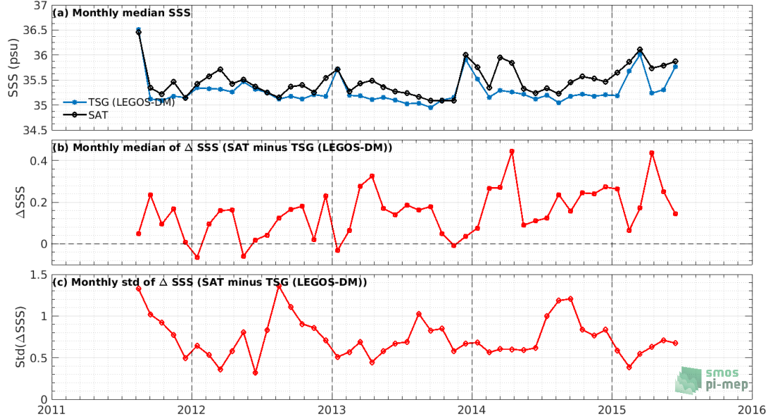
Figure 7: Time series of the monthly median SSS (top), median of \Delta\text{SSS} (Satellite - TSG (LEGOS-DM)) and Std of \Delta\text{SSS} (Satellite - TSG (LEGOS-DM)) over the North Atlantic Ocean Pi-MEP region considering all match-ups collected by the Pi-MEP.
