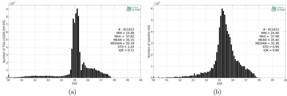
Figure 2: Histograms of SSS from TSG-LEGOS-DM (a) and Aquarius-L3-JPL-V5-7DAY-RUNNING (b) considering all match-up pairs per bins of 0.1 over the North Atlantic Ocean Pi-MEP region and for the full satellite product period.
