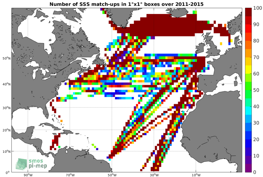
Figure 4: Number of SSS match-ups between TSG-LEGOS-DM SSS and the Aquarius-L3-JPL-V5-7DAY-RUNNING SSS product for the North Atlantic Ocean Pi-MEP region over 1^\circ \times 1^\circ boxes and for the full satellite product period.
