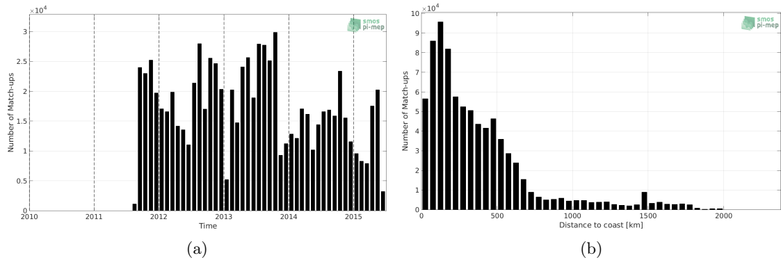
Figure 1: Number of match-ups between TSG-LEGOS-DM and Aquarius-L3-JPL-V5-7DAY-RUNNING SSS as a function of time (a) and as function of the distance to coast (b) over the North Atlantic Ocean Pi-MEP region and for the full satellite product period.
