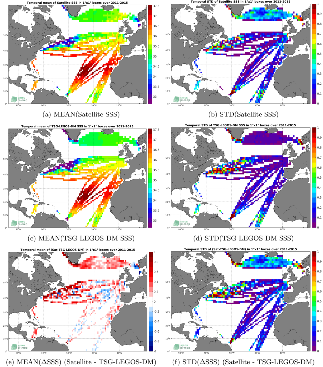
Figure 6: Temporal mean (left) and STD (right) of SSS from Aquarius-L3-JPL-V5-7DAY-RUNNING (top), TSG-LEGOS-DM (middle), and of \Delta SSS (Satellite - TSG-LEGOS-DM). Only match-up pairs are used to generate these maps.
