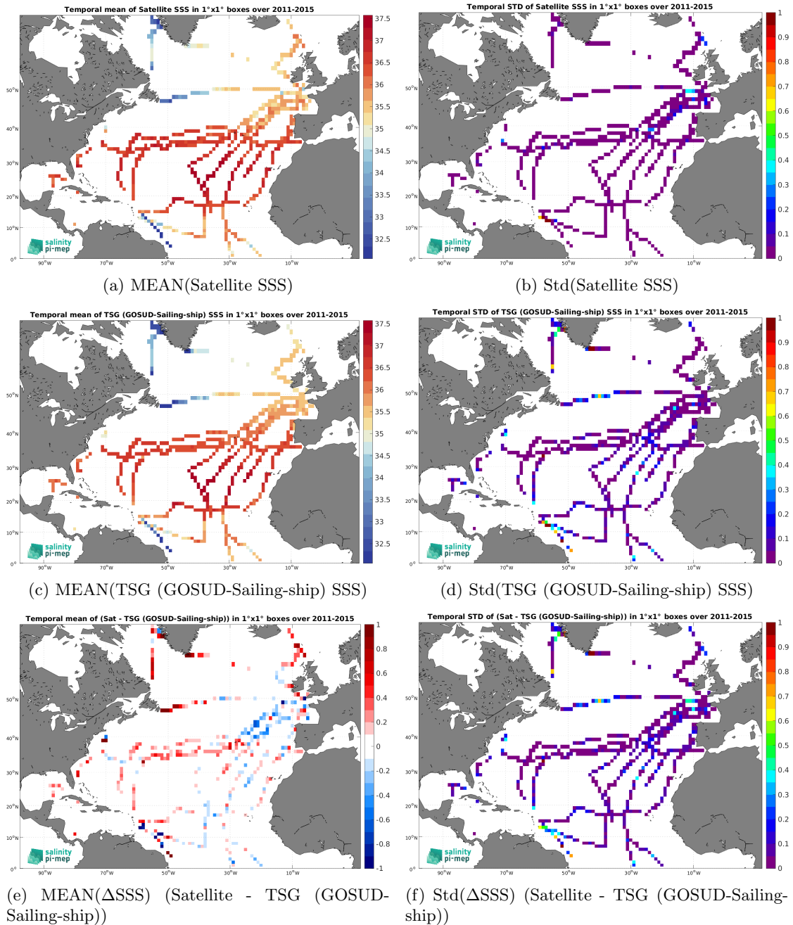
Figure 7: Temporal mean (left) and Std (right) of SSS from Aquarius SSS L3 CAP v5 - 7-Day running (JPL) (top), TSG (GOSUD-Sailing-ship) (middle), and of \Delta SSS (Satellite - TSG (GOSUD-Sailing-ship)). Only match-up pairs are used to generate these maps.
