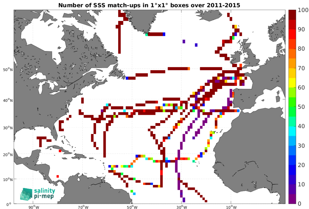
Figure 5: Number of SSS match-ups between TSG (GOSUD-Sailing-ship) SSS and the Aquarius SSS L3 CAP v5 - 7-Day running (JPL) SSS product for the North Atlantic Ocean Pi-MEP region over 1^\circ \times 1^\circ boxes and for the full satellite product period.
