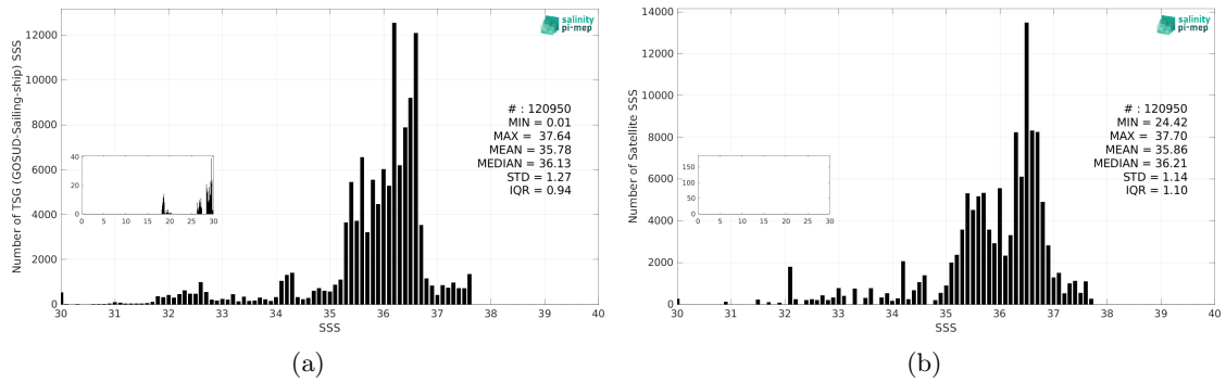
Figure 3: Histograms of SSS from TSG (GOSUD-Sailing-ship) (a) and Aquarius SSS L3 CAP v5 - 7-Day running (JPL) (b) considering all match-up pairs per bins of 0.1 over the North Atlantic Ocean Pi-MEP region and for the full satellite product period.
