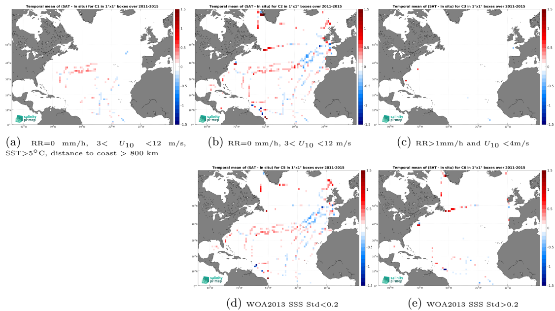
Figure 14: Temporal mean gridded over spatial boxes of size 1^\circ \times 1^\circ of \Delta SSS (Aquarius SSS L3 CAP v5 - 7-Day running (JPL) - TSG (GOSUD-Sailing-ship)) for 5 different subdatasets corresponding to:RR=0 mm/h, 3 < U_{10} < 12 m/s, SST > 5°C, distance to coast > 800 km (a), RR=0 mm/h, 3 < U_{10} < 12 m/s (b), RR > 1mm/h and U_{10} < 4 m/s (c), WOA2013 SSS Std < 0.2 (d), WOA2013 SSS Std > 0.2 (e).
