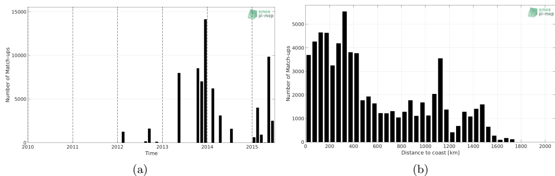
Figure 1: Number of match-ups between TSG-GOSUD-Sailing-ship and Aquarius-L3-JPL-V5-7DAY-RUNNING SSS as a function of time (a) and as function of the distance to coast (b) over the North Atlantic Ocean Pi-MEP region and for the full satellite product period.
