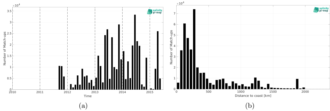
Figure 2: Number of match-ups between TSG (GOSUD-Research-vessel) and Aquarius SSS L3 CAP v5 - 7-Day running (JPL) SSS as a function of time (a) and as function of the distance to coast (b) over the North Atlantic Ocean Pi-MEP region and for the full satellite product period.
