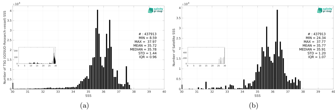
Figure 3: Histograms of SSS from TSG (GOSUD-Research-vessel) (a) and Aquarius SSS L3 CAP v5 - 7-Day running (JPL) (b) considering all match-up pairs per bins of 0.1 over the North Atlantic Ocean Pi-MEP region and for the full satellite product period.
