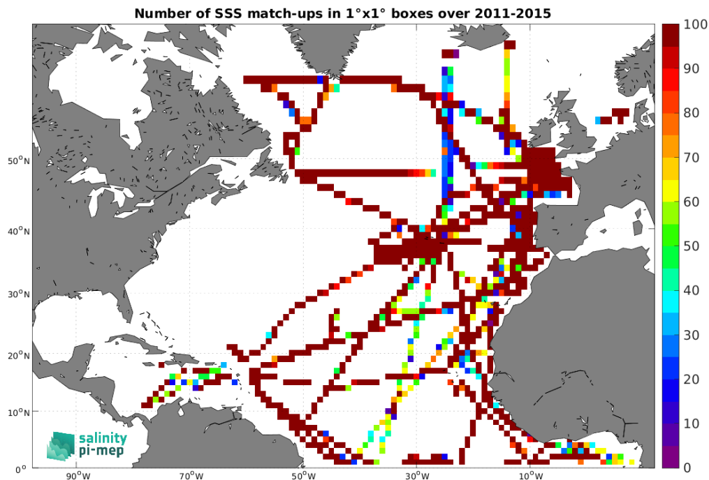
Figure 5: Number of SSS match-ups between TSG (GOSUD-Research-vessel) SSS and the Aquarius SSS L3 CAP v5 - 7-Day running (JPL) SSS product for the North Atlantic Ocean Pi-MEP region over 1^\circ \times 1^\circ boxes and for the full satellite product period.
