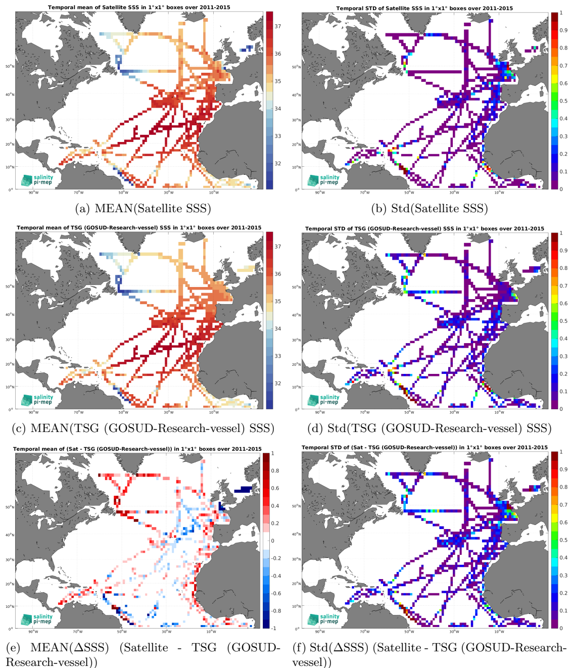
Figure 7: Temporal mean (left) and Std (right) of SSS from Aquarius SSS L3 CAP v5 - 7-Day running (JPL) (top), TSG (GOSUD-Research-vessel) (middle), and of \Delta SSS (Satellite - TSG (GOSUD-Research-vessel)). Only match-up pairs are used to generate these maps.
