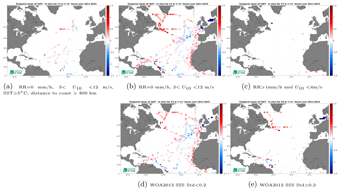
Figure 14: Temporal mean gridded over spatial boxes of size 1^\circ \times 1^\circ of \Delta\text{SSS} (Aquarius SSS L3 CAP v5 - 7-Day running (JPL) - TSG (GOSUD-Research-vessel)) for 5 different subdatasets corresponding to:RR=0 mm/h, 3 < U_{10} < 12 m/s, SST >5^\circ\text{C} , distance to coast > 800 km (a), RR=0 mm/h, 3 < U_{10} < 12 m/s (b), RR >1 mm/h and U_{10} < 4 m/s (c), WOA2013 SSS Std <0.2 (d), WOA2013 SSS Std >0.2 (e).
