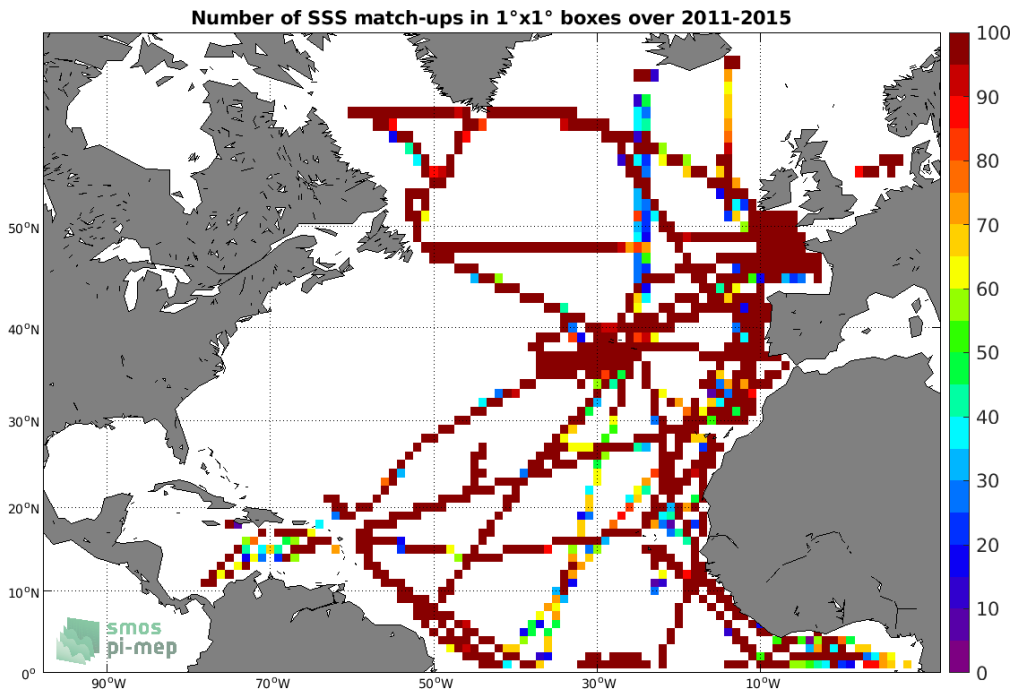
Figure 4: Number of SSS match-ups between TSG (GOSUD-Research-vessel) SSS and the Aquarius SSS L3 CAP v5 - 7-Day running (JPL) SSS product for the North Atlantic Ocean Pi-MEP region over 1^\circ \times 1^\circ boxes and for the full satellite product period.
