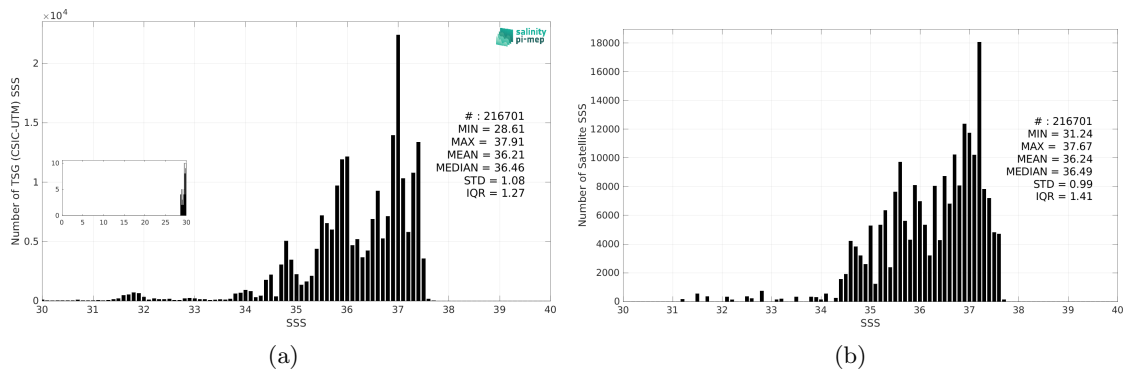
Figure 3: Histograms of SSS from TSG (CSIC-UTM) (a) and Aquarius SSS L3 CAP v5 - 7-Day running (JPL) (b) considering all match-up pairs per bins of 0.1 over the North Atlantic Ocean Pi-MEP region and for the full satellite product period.
