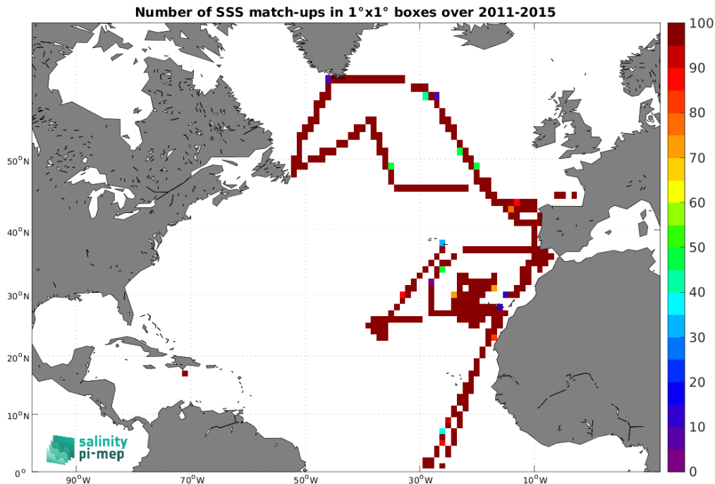
Figure 5: Number of SSS match-ups between TSG (CSIC-UTM) SSS and the Aquarius SSS L3 CAP v5 - 7-Day running (JPL) SSS product for the North Atlantic Ocean Pi-MEP region over 1^\circ \times 1^\circ boxes and for the full satellite product period.
