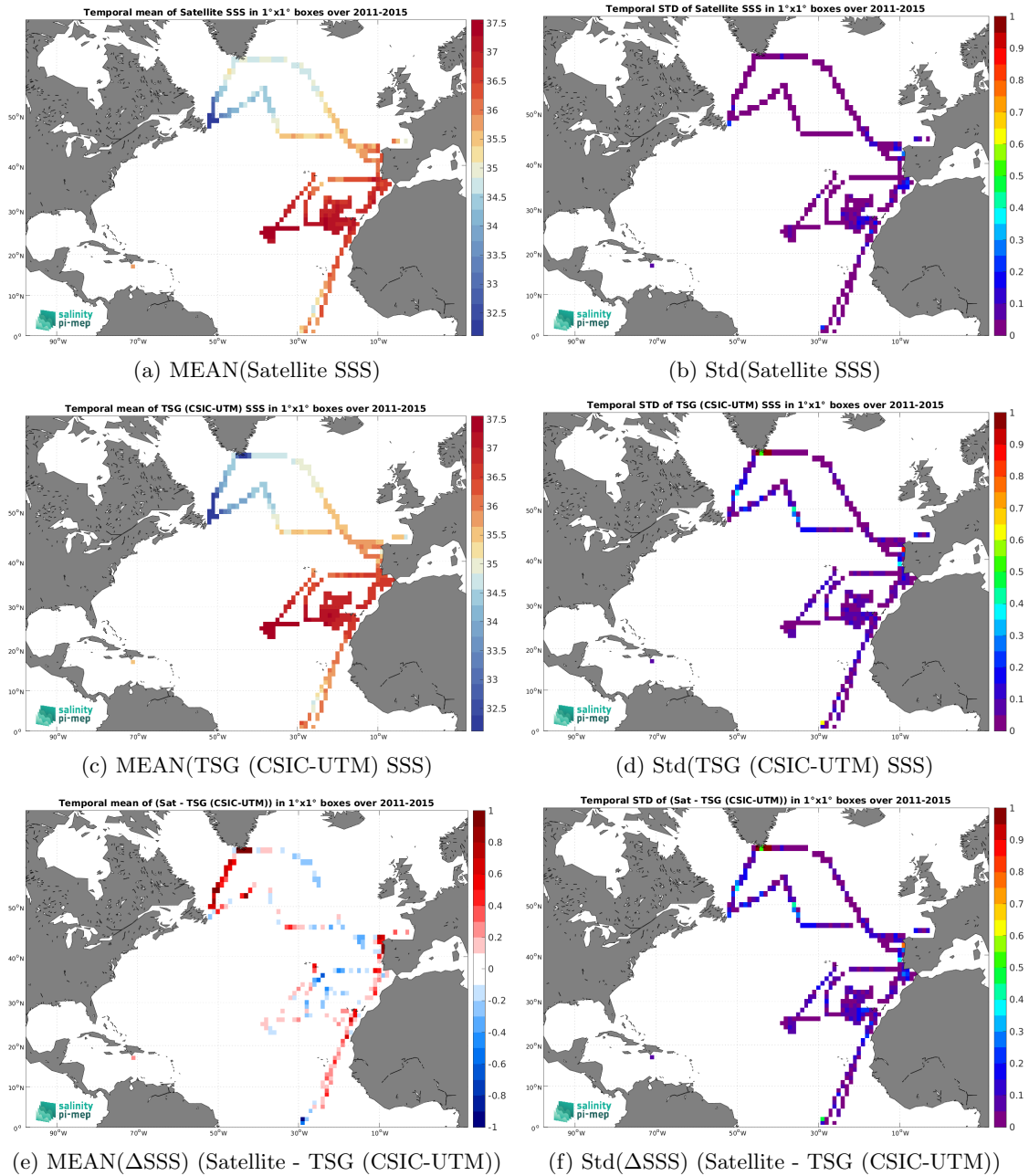
Figure 7: Temporal mean (left) and Std (right) of SSS from Aquarius SSS L3 CAP v5 - 7-Day running (JPL) (top), TSG (CSIC-UTM) (middle), and of \Delta SSS (Satellite - TSG (CSIC-UTM)). Only match-up pairs are used to generate these maps.
