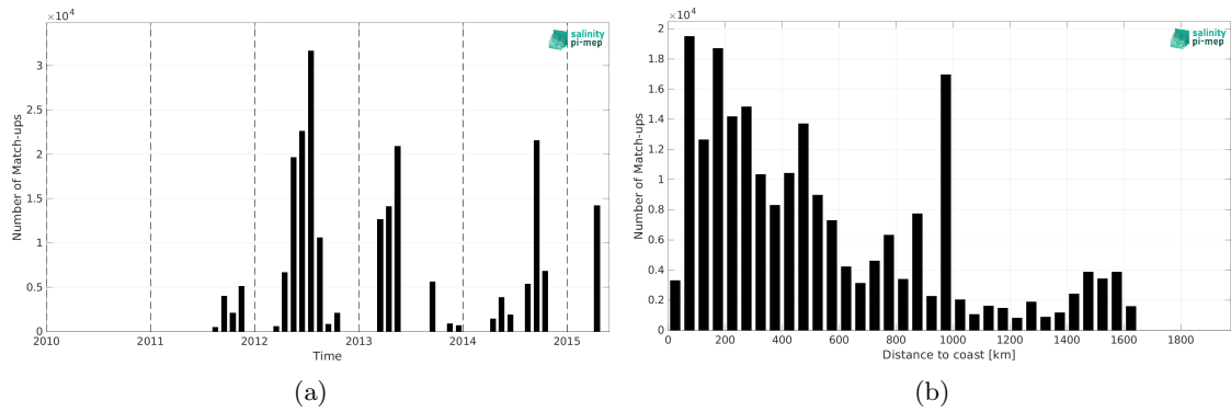
Figure 2: Number of match-ups between TSG (CSIC-UTM) and Aquarius SSS L3 CAP v5 - 7-Day running (JPL) SSS as a function of time (a) and as function of the distance to coast (b) over the North Atlantic Ocean Pi-MEP region and for the full satellite product period.
