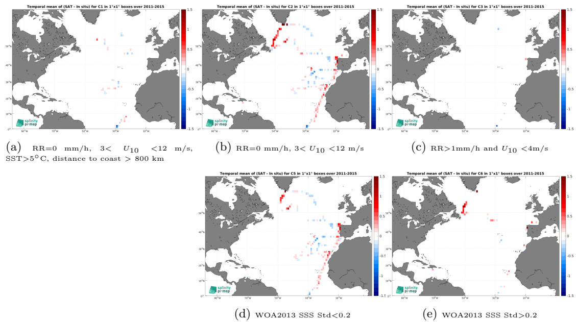
Figure 14: Temporal mean gridded over spatial boxes of size 1^\circ \times 1^\circ of \Delta\text{SSS} (Aquarius SSS L3 CAP v5 - 7-Day running (JPL) - TSG (CSIC-UTM)) for 5 different subdatasets corresponding to:RR=0 mm/h, 3 < U_{10} < 12 m/s, SST >5^\circ\text{C} , distance to coast > 800 km (a), RR=0 mm/h, 3 < U_{10} < 12 m/s (b), RR >1 mm/h and U_{10} < 4 m/s (c), WOA2013 SSS Std <0.2 (d), WOA2013 SSS Std >0.2 (e).
