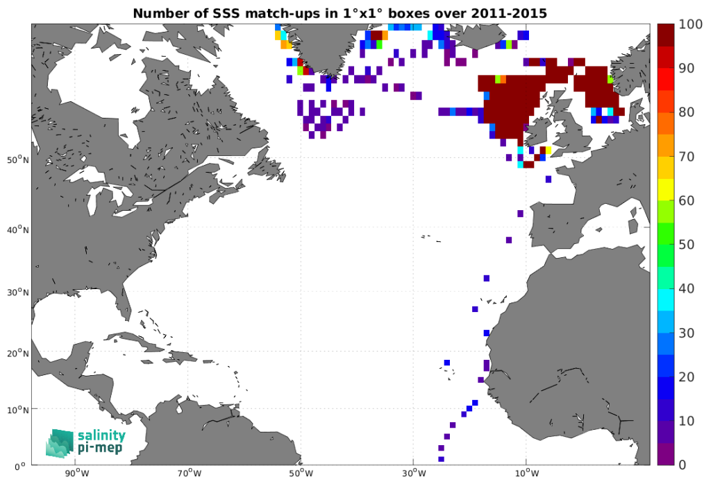
Figure 5: Number of SSS match-ups between ICES SSS and the Aquarius SSS L3 CAP v5 - 7-Day running (JPL) SSS product for the North Atlantic Ocean Pi-MEP region over 1^\circ \times 1^\circ boxes and for the full satellite product period.
