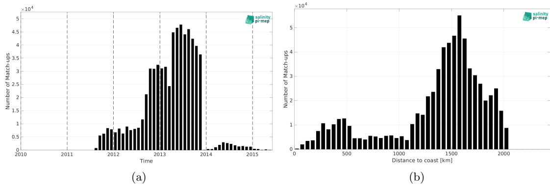
Figure 2: Number of match-ups between Surface drifters and Aquarius SSS L3 CAP v5 - 7-Day running (JPL) SSS as a function of time (a) and as function of the distance to coast (b) over the North Atlantic Ocean Pi-MEP region and for the full satellite product period.
