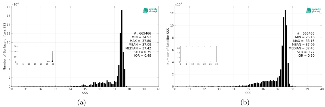
Figure 3: Histograms of SSS from Surface drifters (a) and Aquarius SSS L3 CAP v5 - 7-Day running (JPL) (b) considering all match-up pairs per bins of 0.1 over the North Atlantic Ocean Pi-MEP region and for the full satellite product period.
