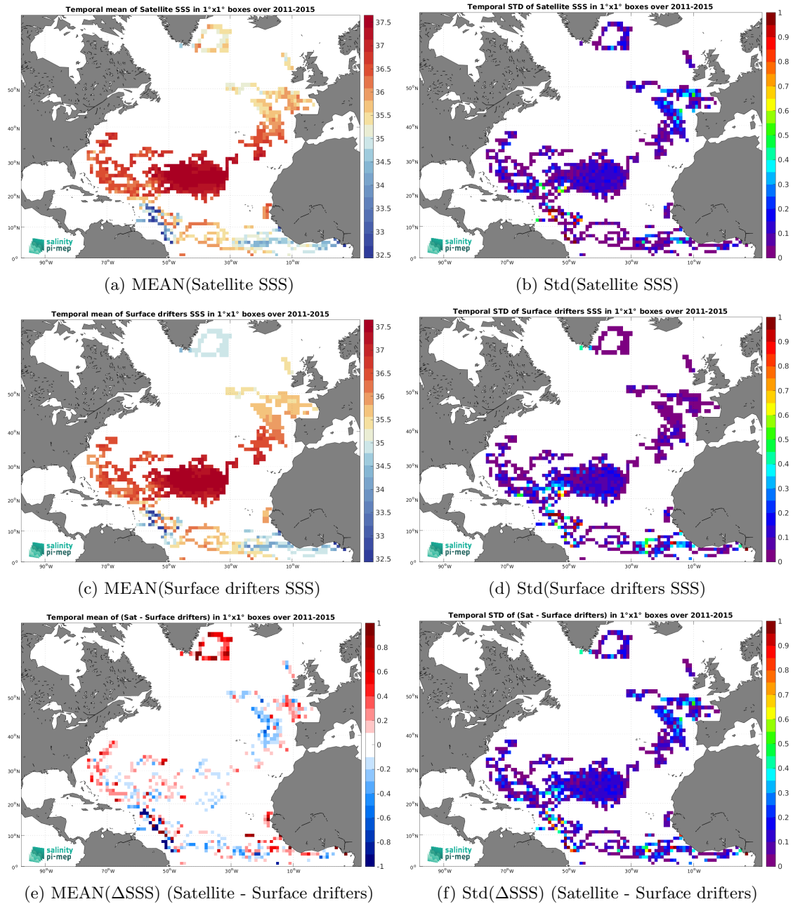
Figure 6: Temporal mean (left) and Std (right) of SSS from Aquarius SSS L3 CAP v5 - 7-Day running (JPL) (top), Surface drifters (middle), and of \Delta SSS (Satellite - Surface drifters). Only match-up pairs are used to generate these maps.
