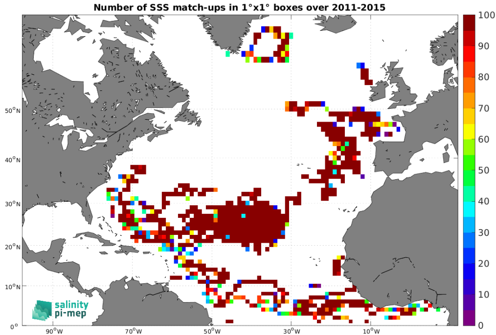
Figure 4: Number of SSS match-ups between Surface drifters SSS and the Aquarius SSS L3 CAP v5 - 7-Day running (JPL) SSS product for the North Atlantic Ocean Pi-MEP region over 1^\circ \times 1^\circ boxes and for the full satellite product period.
