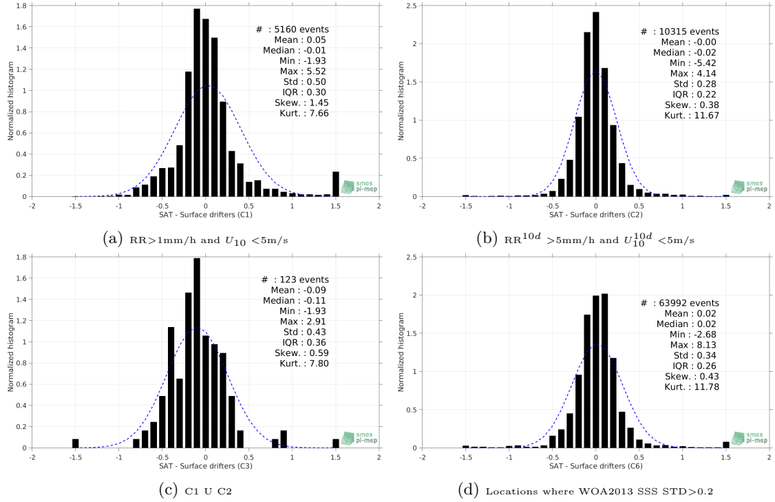
Figure 12: Normalized histogram of \Delta SSS (Aquarius-L3-JPL-V5-7DAY-RUNNING - Surface drifters) for 6 different subdatasets corresponding to: RR > 1mm/h and U_{10} < 5 m/s (a), RR^{10d} > 5 mm/h and U_{10}^{10d} < 5 m/s (b), C1 U C2 (c), Locations where WOA2013 SSS STD > 0.2 (d).
