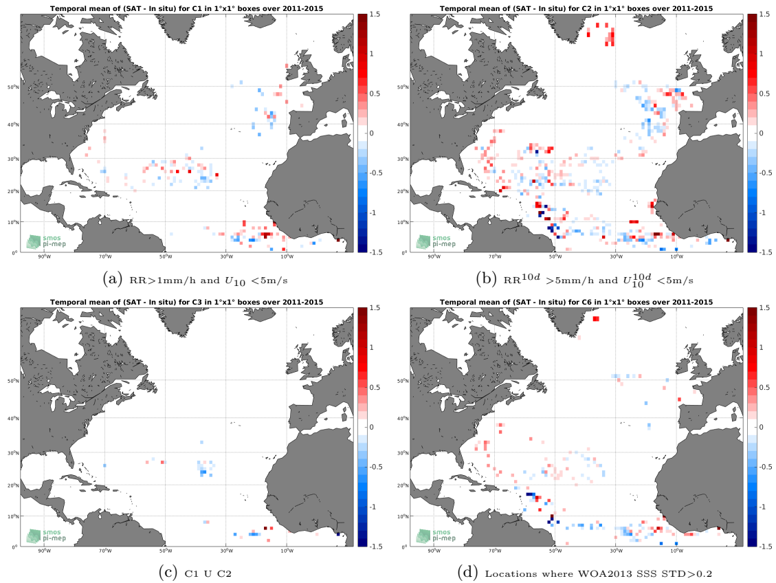
Figure 11: Temporal mean gridded over spatial boxes of size 1^\circ \times 1^\circ of \Delta SSS (Aquarius-L3-JPL-V5-7DAY-RUNNING - Surface drifters) for 4 different subdatasets corresponding to: RR > 1\text{mm/h} and U_{10} < 5\text{m/s} (a), RR^{10d} > 5\text{mm/h} and U_{10}^{10d} < 5\text{m/s} (b), C1 U C2 (c), Locations where WOA2013 SSS STD > 0.2 (d).
