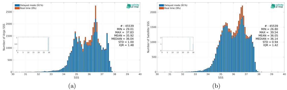
Figure 3: Histograms of SSS from Argo (a) and Aquarius SSS L3 CAP v5 - 7-Day running (JPL) (b) considering all match-up pairs per bins of 0.1 over the North Atlantic Ocean Pi-MEP region and for the full satellite product period.
