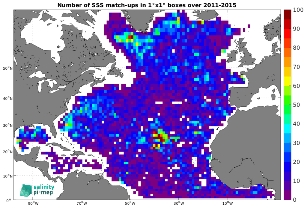
Figure 5: Number of SSS match-ups between Argo SSS and the Aquarius SSS L3 CAP v5 - 7-Day running (JPL) SSS product for the North Atlantic Ocean Pi-MEP region over 1^\circ \times 1^\circ boxes and for the full satellite product period.
