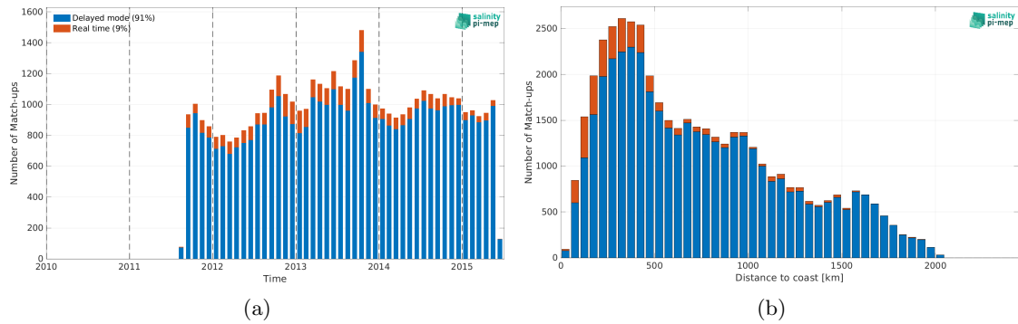
Figure 2: Number of match-ups between Argo and Aquarius SSS L3 CAP v5 - 7-Day running (JPL) SSS as a function of time (a) and as function of the distance to coast (b) over the North Atlantic Ocean Pi-MEP region and for the full satellite product period.
